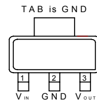
SOT-223 (Top View) APL5509R
