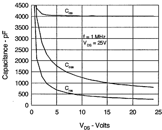
Fig.9 Capacitance Curves
