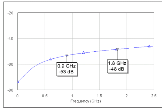
TX2-ANT Isolation
