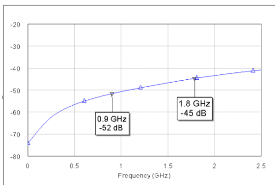
TX1-ANT Isolation
