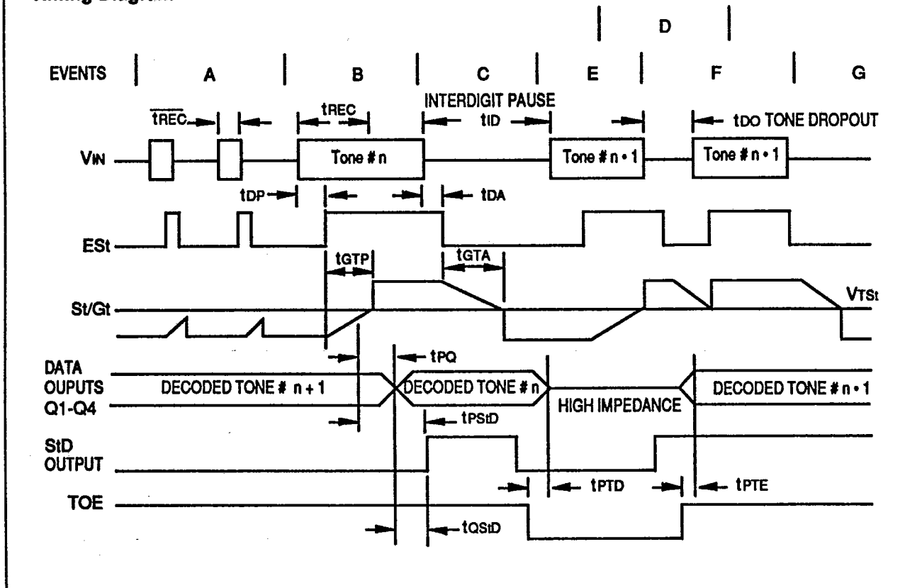
Timing Diagram
