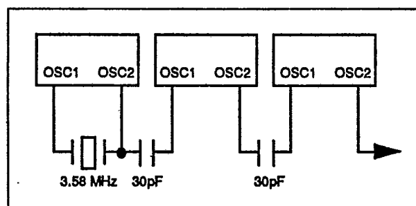
Figure 7. CM8870C Crystal Connection
