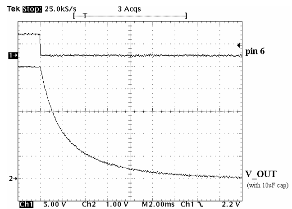
Figure 16. LDO Power-Down
