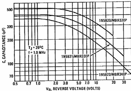
FIGURE 11 – TYPICAL CAPACITANCE
