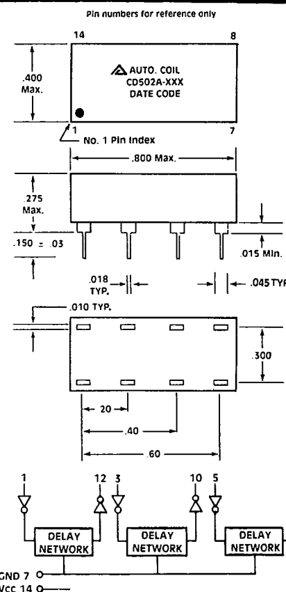
14 PIN DIP
