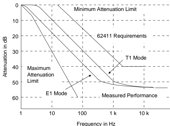
Figure 17. Typical Jitter Transfer Function
