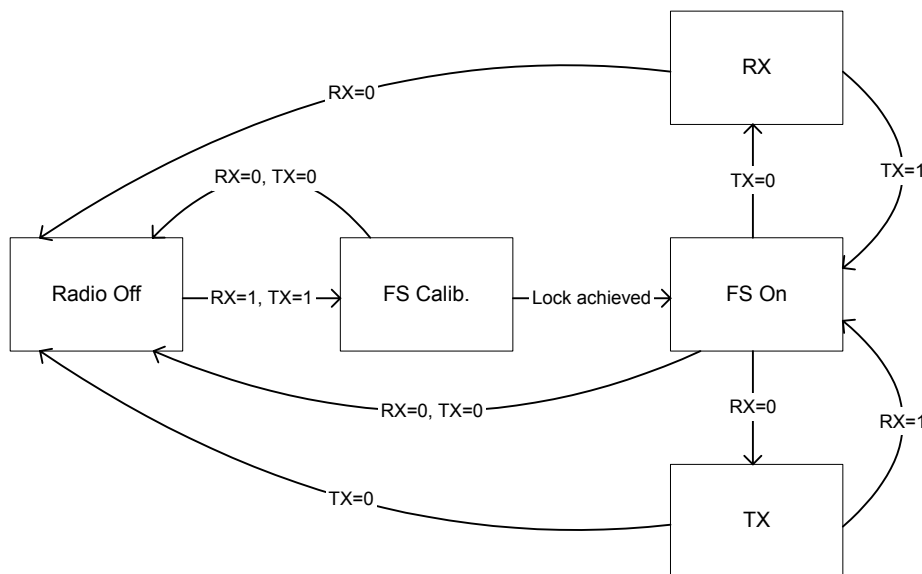
Figure 14. Radio control state diagram using the RX and TX pins
