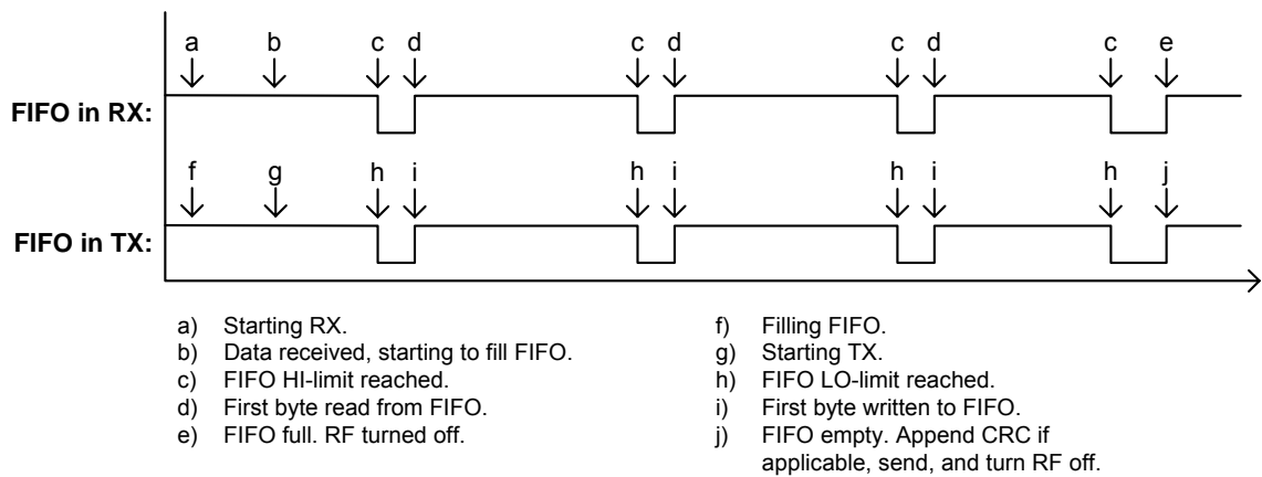
Figure 10. FIFO pin timing diagram
