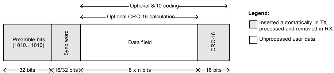
Figure 17. Packet format details (with recommended lengths of preamble and synchronization word)
