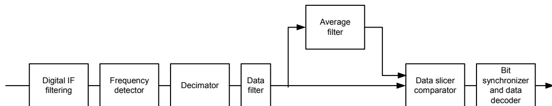
Figure 19. Demodulator block diagram
