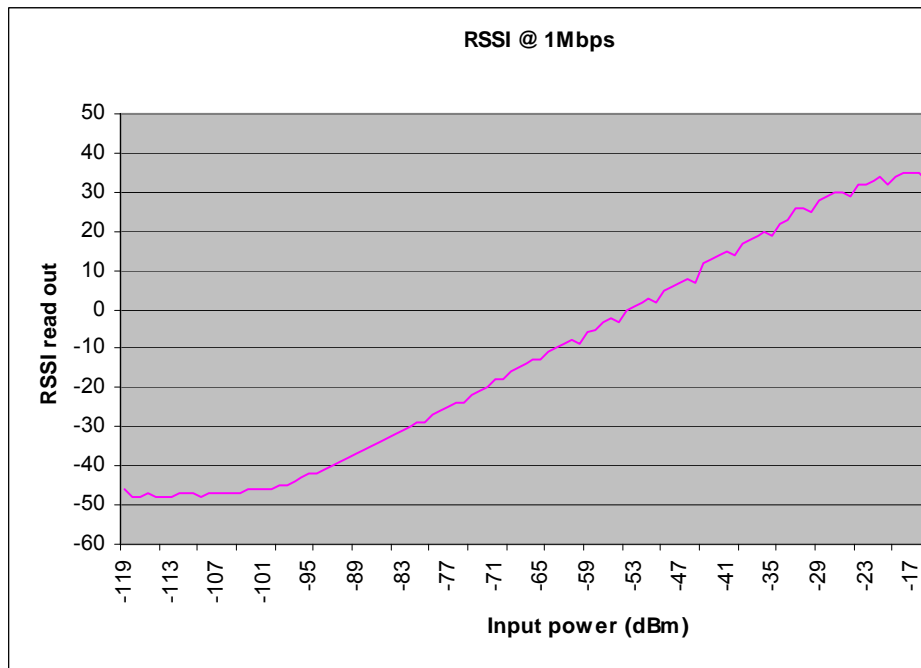
Figure 20. Typical RSSI value vs. input power
