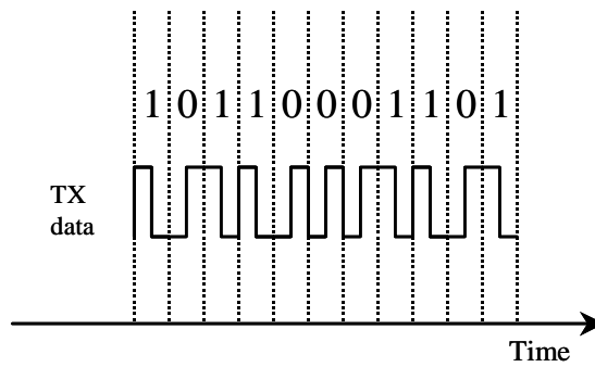
Figure 13. Manchester encoding
