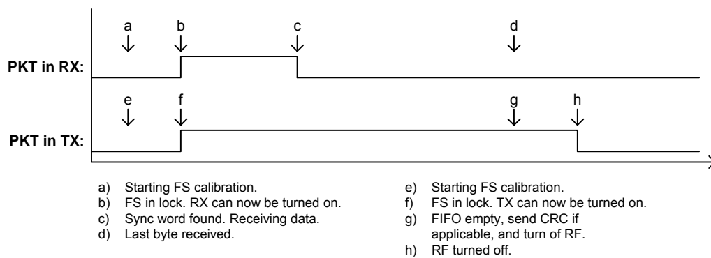
Figure 18. PKT pin timing diagram
