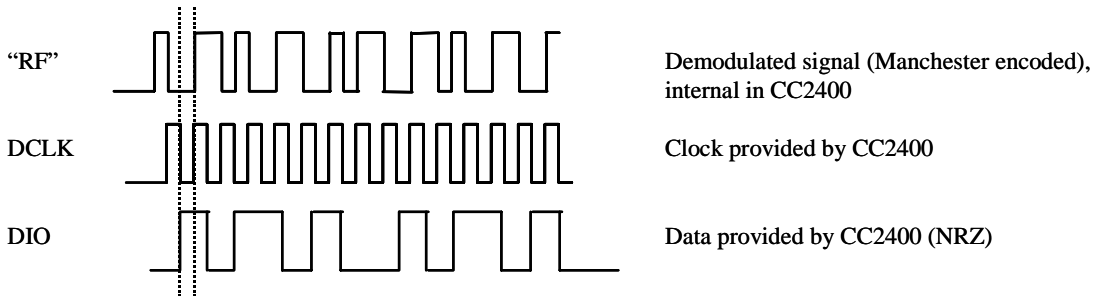
Figure 12. Synchronous Manchester encoded mode
