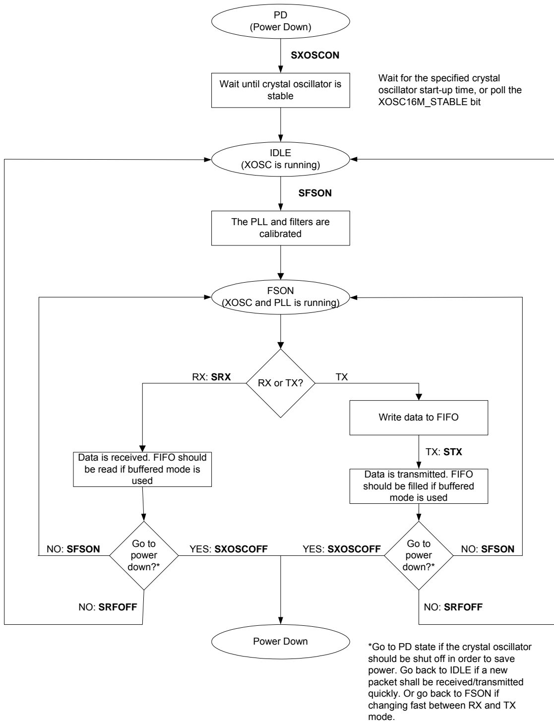
Figure 16. Sequence for activating RX or TX mode
