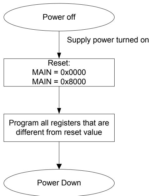
Figure 15. Initializing sequence
