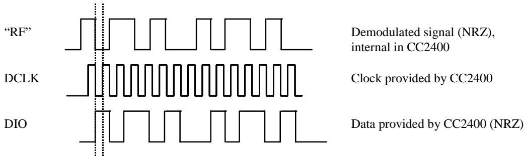
Figure 11. Synchronous NRZ mode
