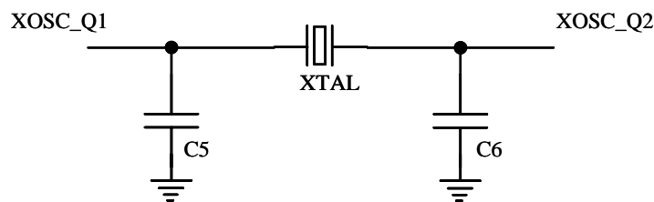
Figure 21. Crystal oscillator circuit
