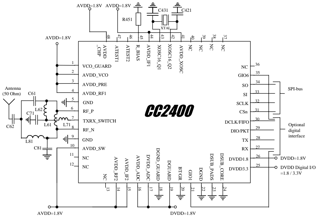
Figure 3 Typical application circuit with discrete balun for single-ended operation
