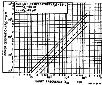
Fig. 13 - Dynamic power dissipation.
