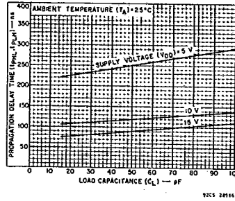
Fig. 12 - Typical propagation delay time as a function of load capacitance.
