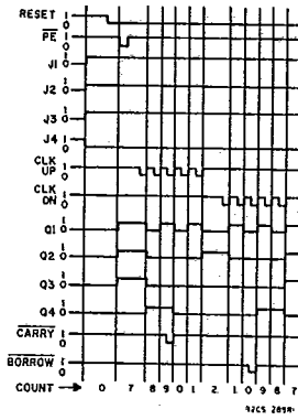
Fig. 3 - CD40192B timing diagram.
