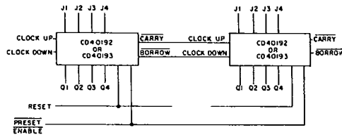
Fig. 18 - Cascaded counter packages.
