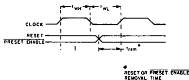
Fig. 10 - Timing diagram defining t rem
