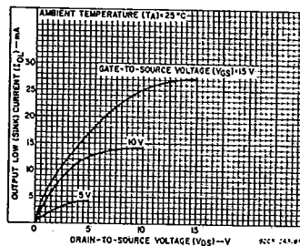
Fig. 6 - Typical output low (sink) current characteristics.
