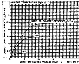
Fig. 7 - Minimum output low (sink) current characteristics.
