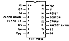
CD40192B, CD40193B TERMINAL ASSIGNMENT
