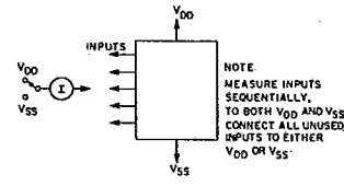
Fig. 17 - Input current test circuit.
