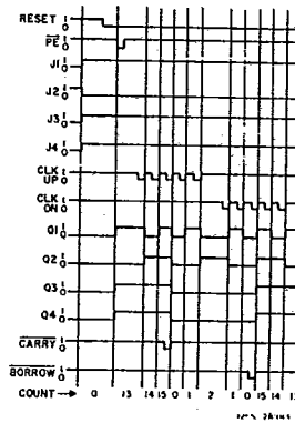
Fig. 5 - CD40193B timing diagram.
