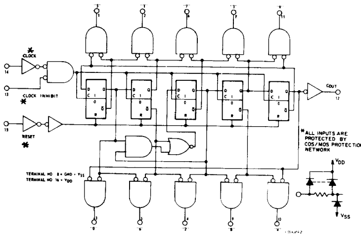
Fig. 1 - Logic diagram.
