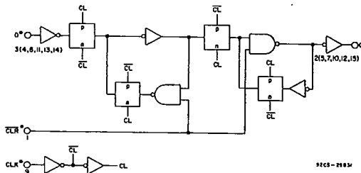
Fig. 1 - Logic diagram (1 of 6 flip-flops).
