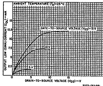
Fig. 4— Minimum output low (sink) current characteristics.
