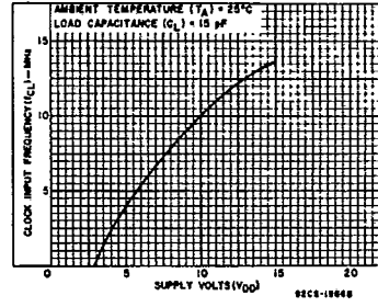
Fig. 8 - Typical maximum clock input frequency vs. V DD .
