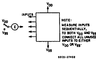
Fig. 11 - Input leakage test circuit.
