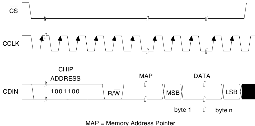
Figure 15. Control Port Timing, SPI Format (Write)
