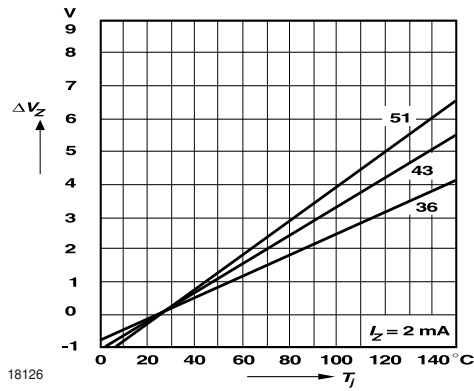
Figure 13. Change of Zener voltage versus junction temperature
