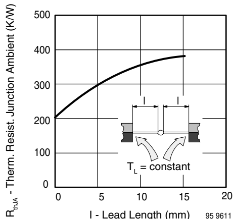
Fig. 1 - Thermal Resistance vs. Lead Length
