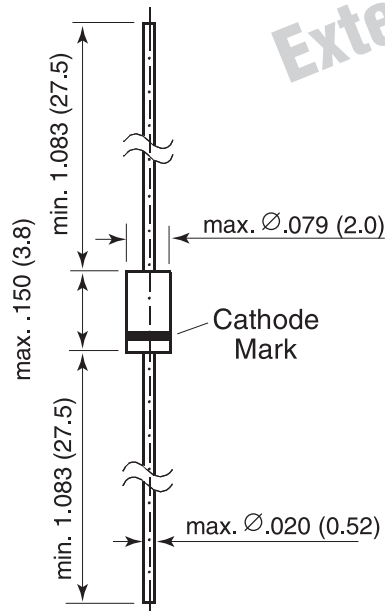
DO-204AH (DO-35 Glass)
