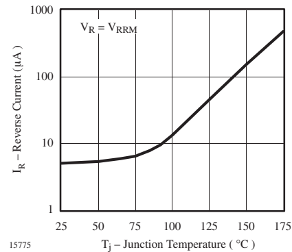
Figure 3. Max. Reverse Current vs. Junction Temperature
