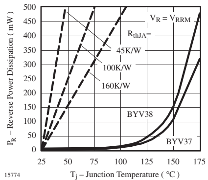
Figure 2. Max. Reverse Power Dissipation vs. Junction Temperature
