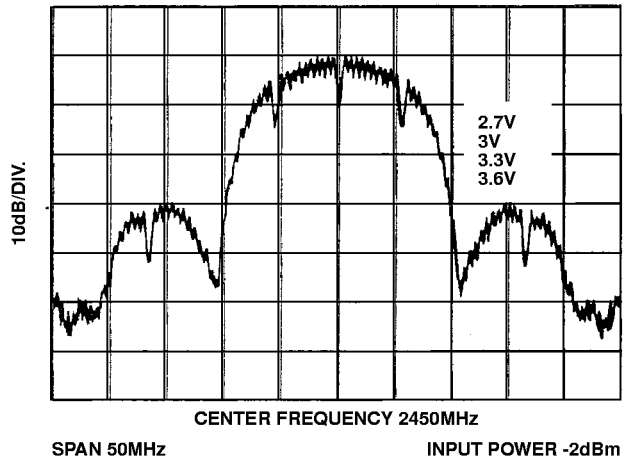
FIGURE 9. DSSS OUTPUT SIGNAL OVER VOLTAGE
