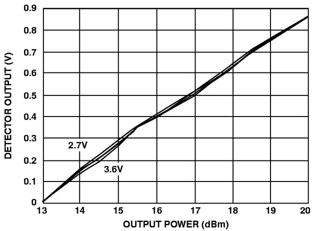
FIGURE 11. DETECTOR OUTPUT OVER VOLTAGE
