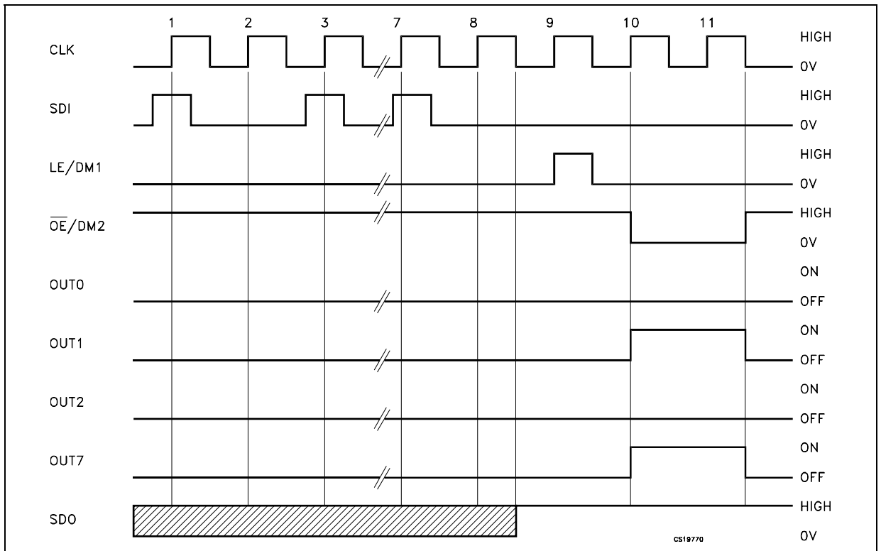
Figure 7: Timing Diagram
