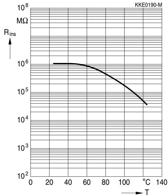
Insulation resistance R_{\text{ins}} versus temperature T
