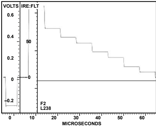
Figure 131. NTSC Luma
