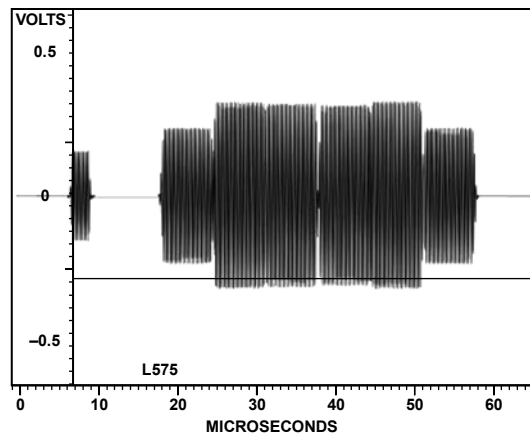
Figure 135. PAL Chroma
