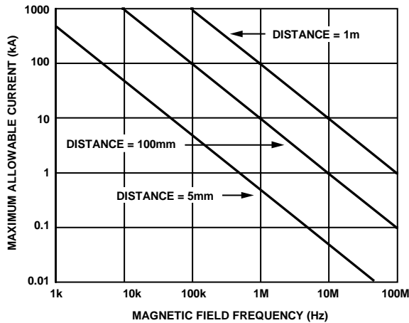
Figure 14. Maximum Allowable Current for Various Current-to-ADuM120x Spacings
