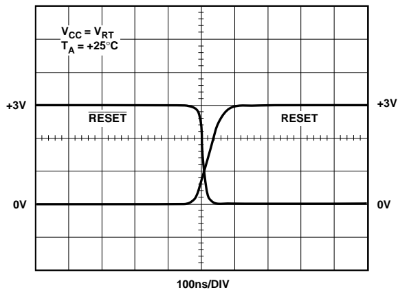
Figure 12. \overline{\text{RESET}} , \text{RESET} Assertion
