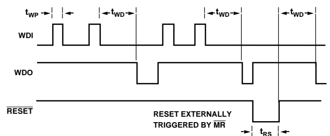
Figure 4. Watchdog Timing
