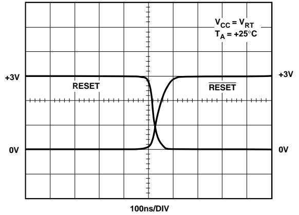
Figure 13. \overline{\text{RESET}} , \text{RESET} Deassertion
