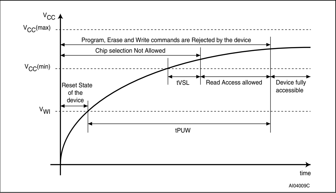
Figure 20. Power-up timing
