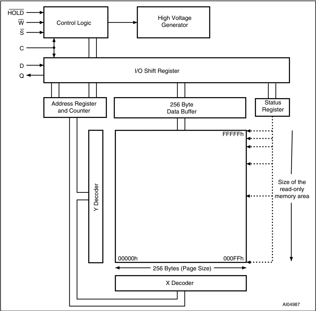
Figure 6. Block diagram
