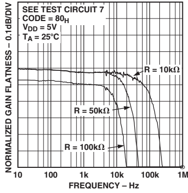
TPC 19. Normalized Gain Flatness vs. Frequency
