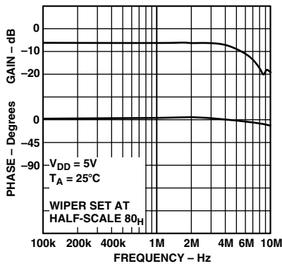
TPC 25. 1 kΩ Gain and Phase vs. Frequency
