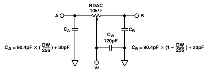
Figure 8. RDAC Circuit Simulation Model for RDAC = 10 k \Omega
