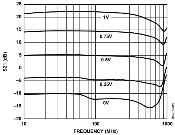
Figure 3. Frequency Response vs. V_{GAIN}
