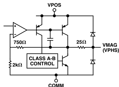
Circuit B
