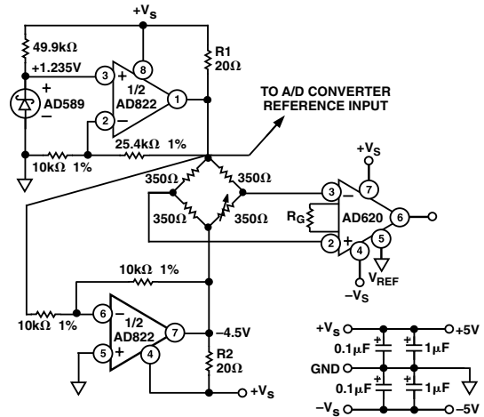
Figure 10. Low Dropout Bipolar Bridge Driver
