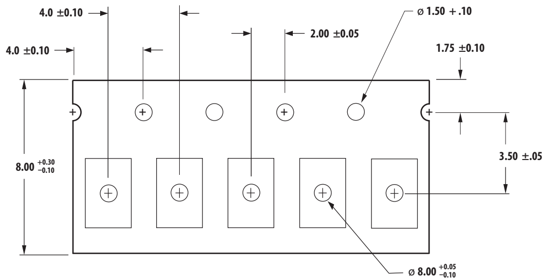
Figure 30. SMD Tape Packing.
