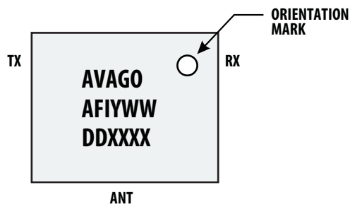
Figure 29. Product Marking and Pin Orientation.
