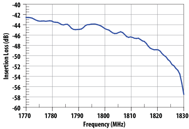
Figure 15. Ant-Rx Rejection, 1770-1830 MHz.
