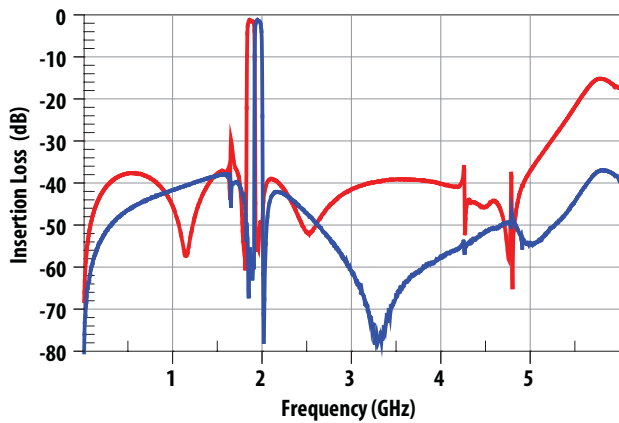
Figure 7. Tx-Ant and Ant-Rx Wideband Insertion Loss.
