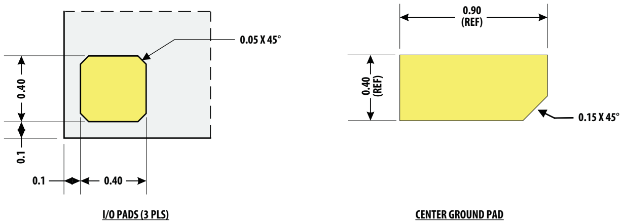
Figure 21. Pad Detail.
