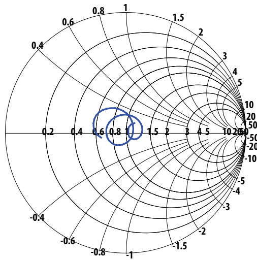
Figure 17. Rx Port Impedance in Rx Band.
