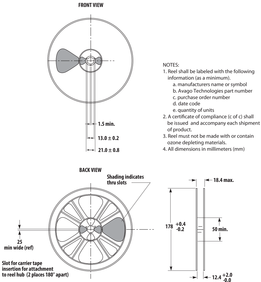
Figure 32. SMT Reel Drawing.
