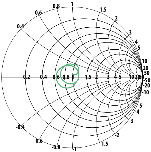
Figure 18. Ant Port Impedance in Tx Band.
