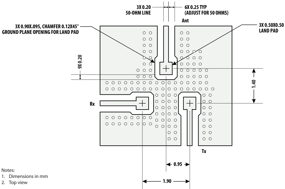
Figure 22. Suggested PCB Layout.
