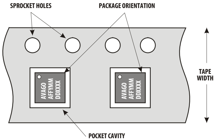
Figure 31. Unit Orientation in SMT Tape.
