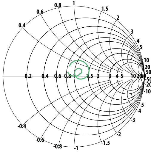
Figure 19. Ant Port Impedance in Rx Band.
