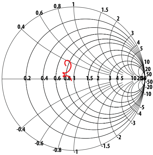
Figure 16. Tx Port Impedance in Tx Band.
