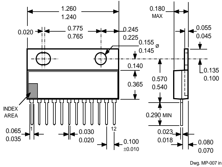
A3952SW Dimensions in Inches (controlling dimensions)
