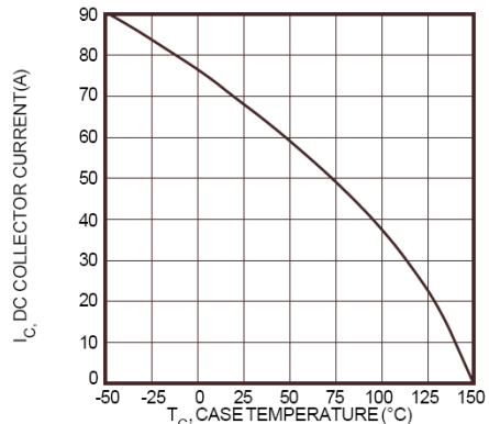
FIGURE 8, DC Collector Current vs Case Temperature
