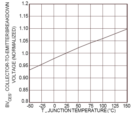
FIGURE 7, Breakdown Voltage vs. Junction Temperature
