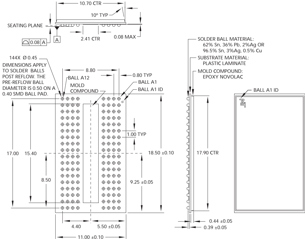
Figure 5: 144-Ball \mu BGA
