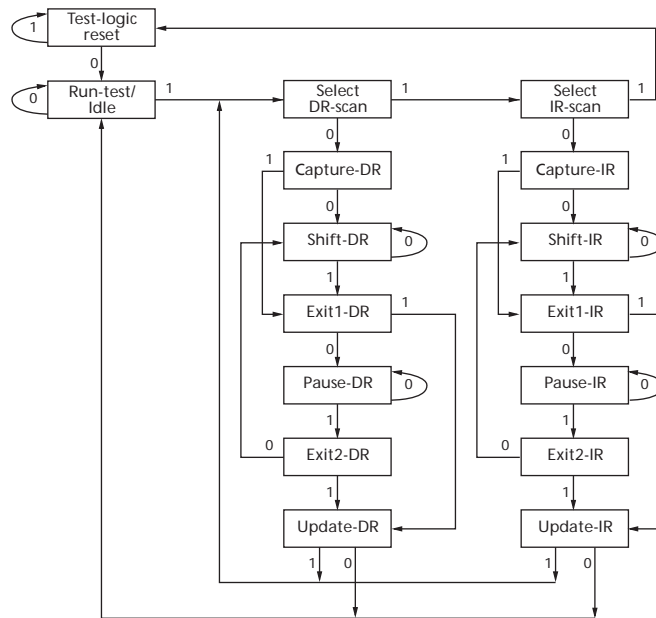
Figure 42: TAP Controller Block Diagram
