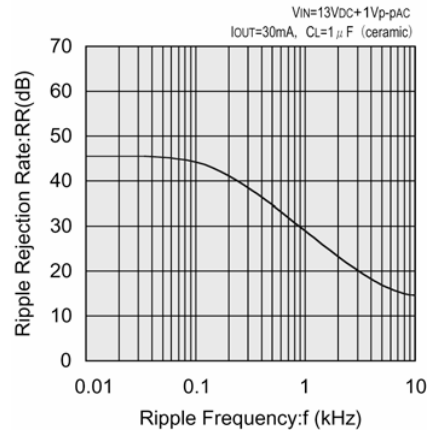
XC6202PC02 (12V)
