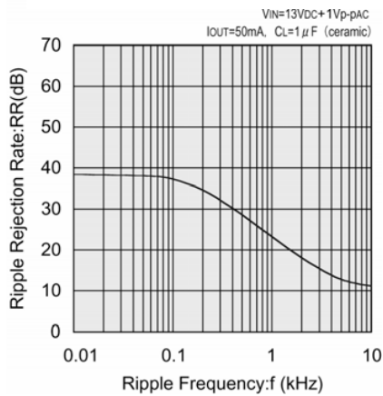
XC6202PC02 (12V)
