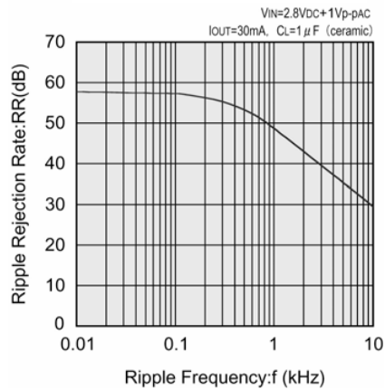
XC6202P182 (1.8V)
