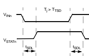
OVER TEMP STATUS TIMING
