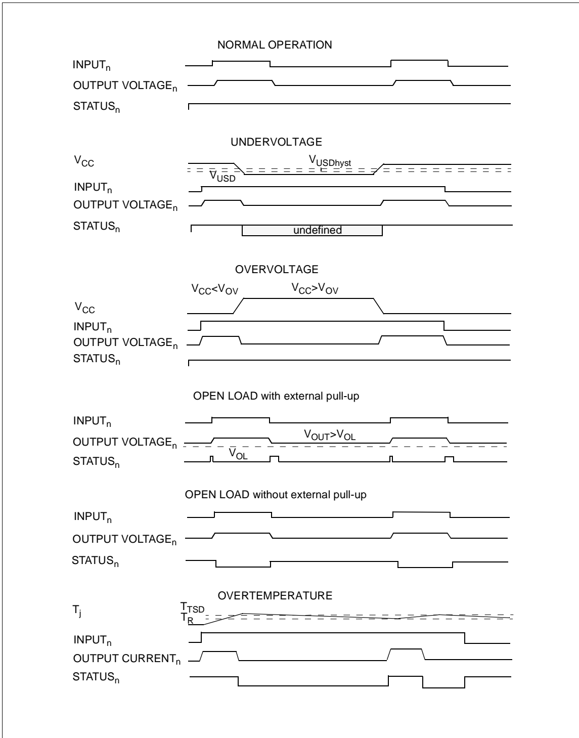
Figure 1: Waveforms
