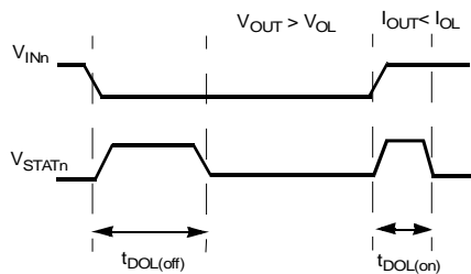
OPEN LOAD STATUS TIMING (with external pull-up)
