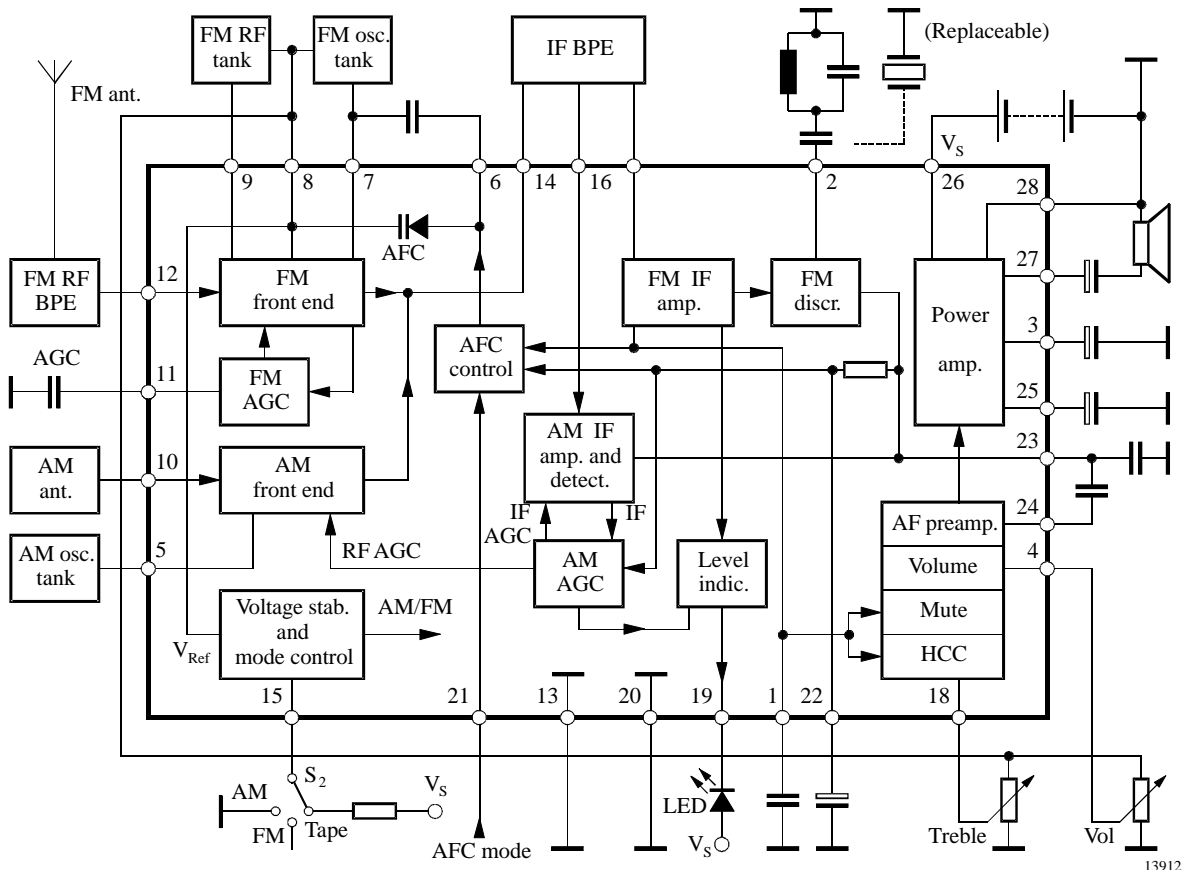
Figure 1. Block diagram
