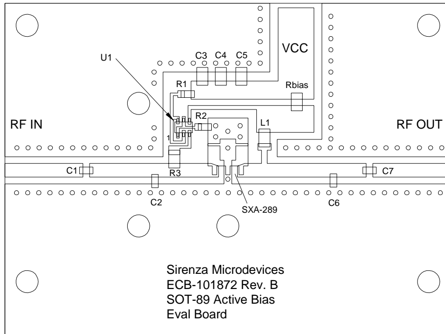
Active Bias Evaluation Board Layout
