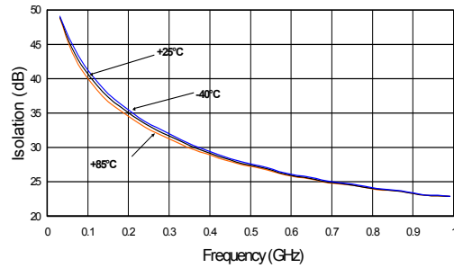
Isolation, 1000 pF
