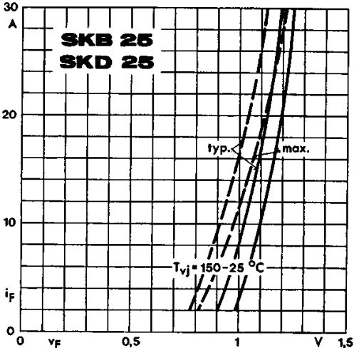
Fig. 9 Forward characteristics of a single diode
