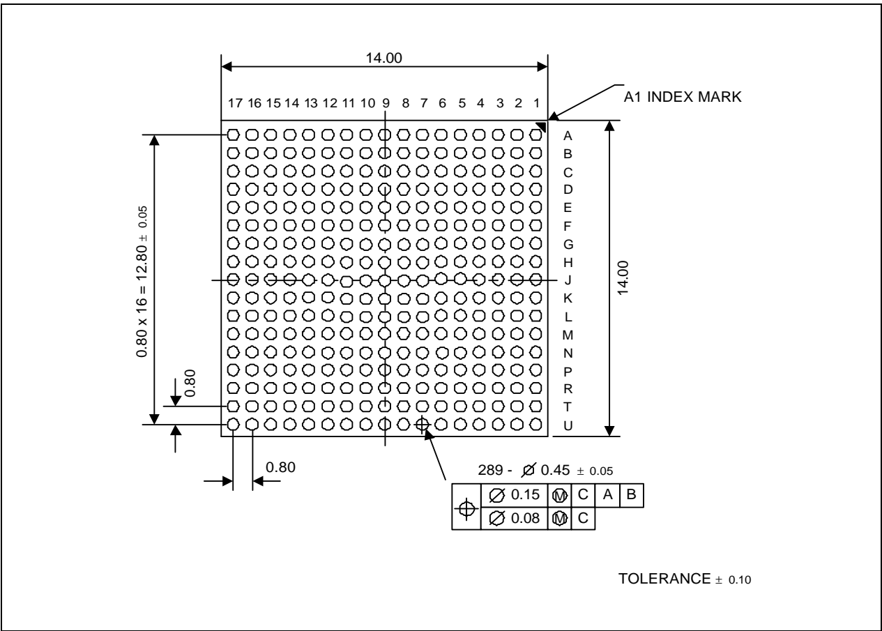
Figure 26-2. 289-FBGA-1414 Package Dimension 2 (Bottom View)
