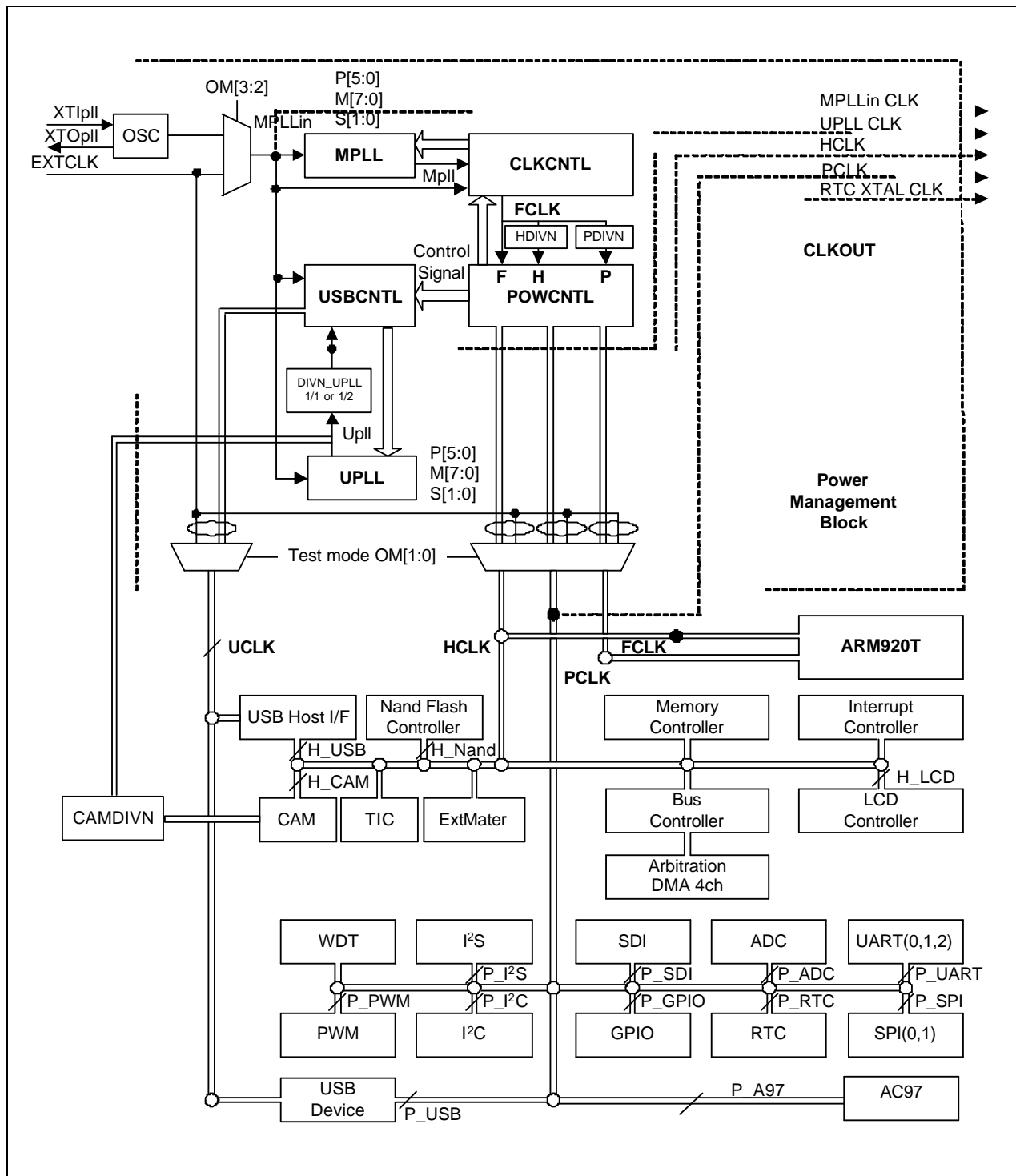
Figure 7-1. Clock Generator Block Diagram
