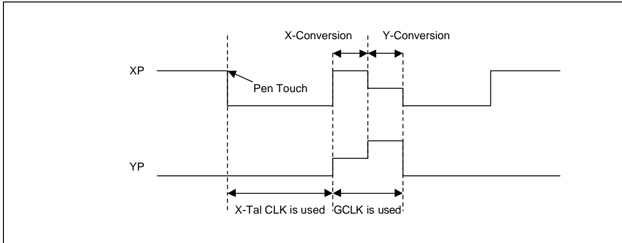
Figure 16-2. ADC and Touch Screen Operation signal
