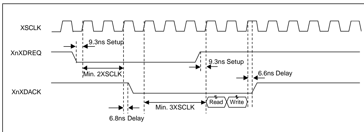
Figure 8-1. Basic DMA Timing Diagram
