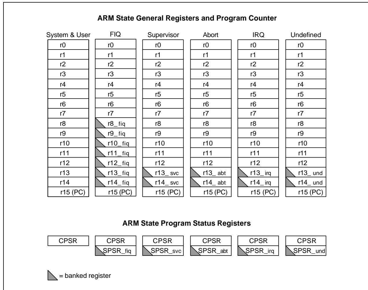
Figure 2-3. Register Organization in ARM State
