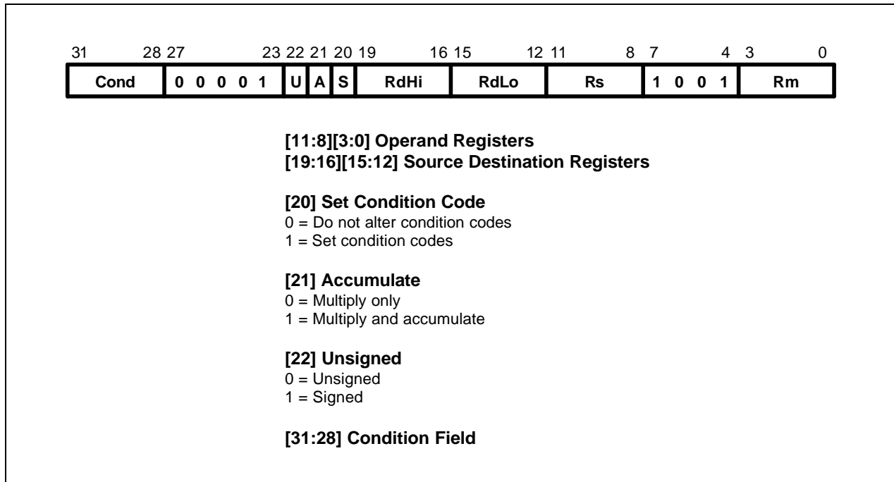
Figure 3-13. Multiply Long Instructions
