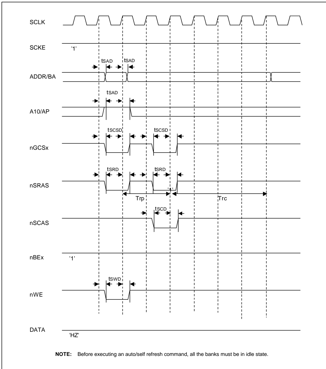
Figure 27-25. SDRAM Auto Refresh Timing Diagram (Trp=2, Trc=4)
