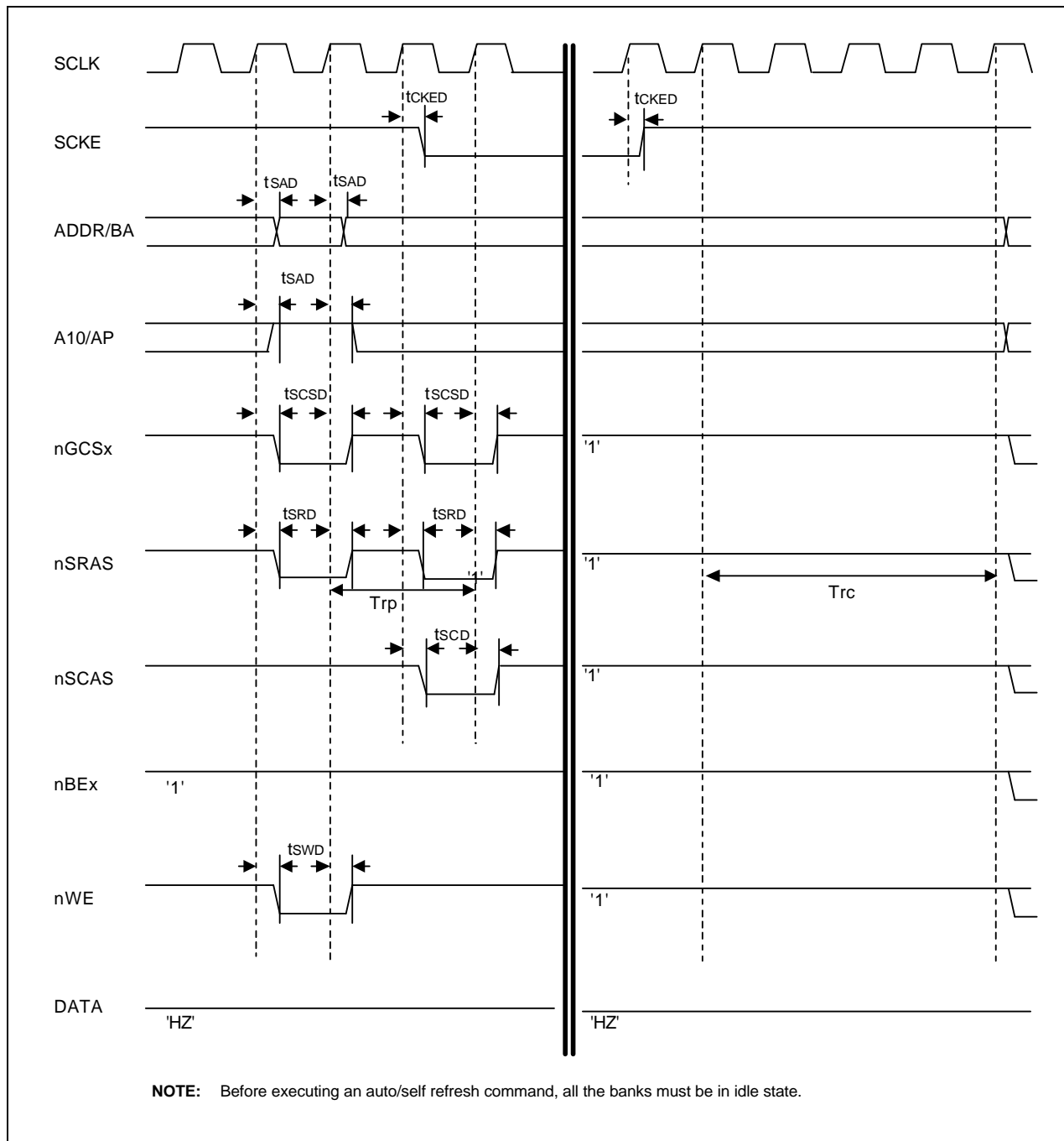
Figure 27-27. SDRAM Self Refresh Timing Diagram ( Trp=2 , Trc=4 )
