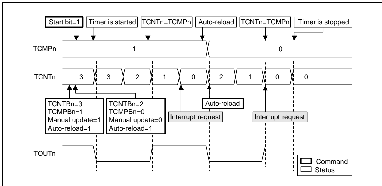
Figure 10-2. Timer Operations
