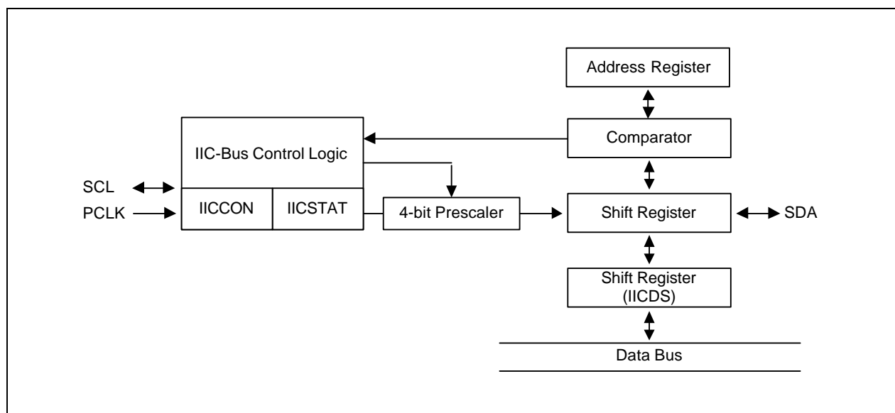
Figure 20-1. IIC-Bus Block Diagram
