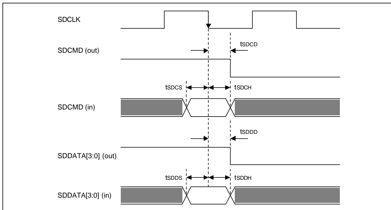
Figure 27-34. SD/MMC Interface Timing Diagram
