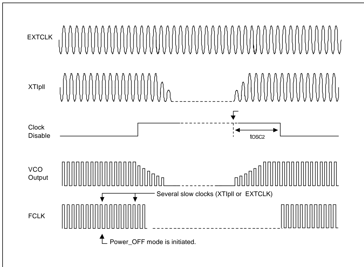
Figure 27-8. Sleep Mode Return Oscillation Setting Timing Diagram
