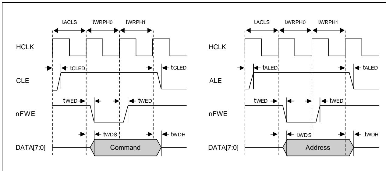
Figure 27-36. NAND Flash Address/Command Timing Diagram
