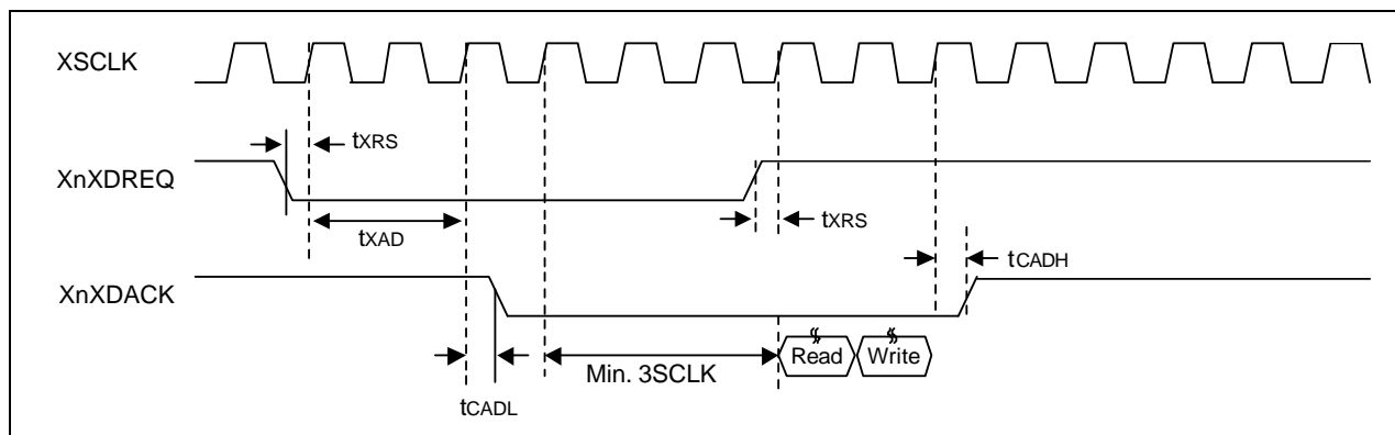
Figure 27-30. External DMA Timing Diagram (Handshake, Single transfer)
