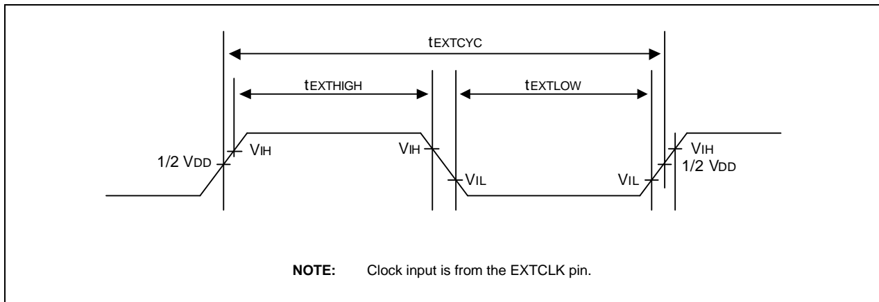
Figure 27-3. EXTCLK Clock Input Timing Diagram
