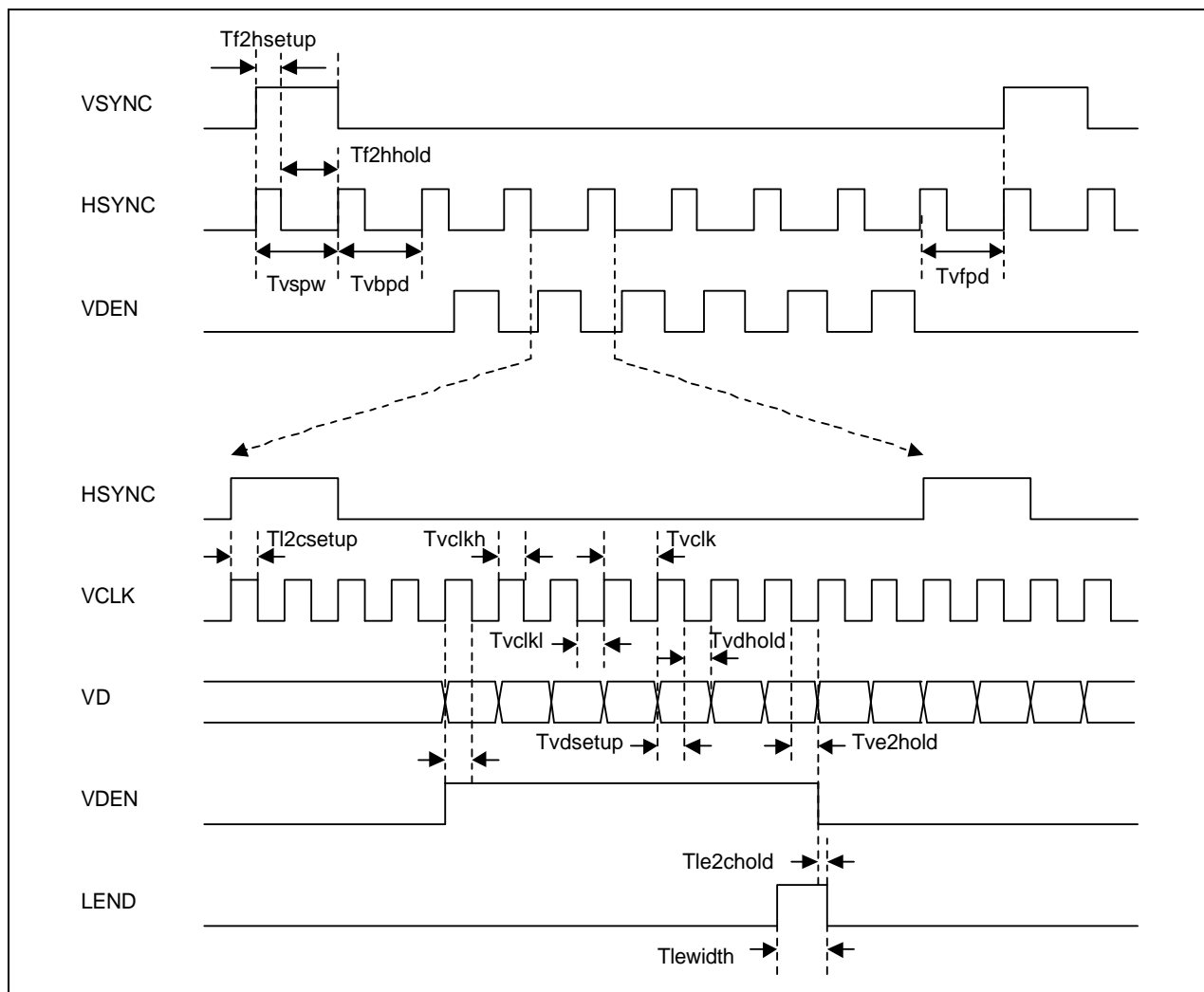
Figure 27-31. TFT LCD Controller Timing Diagram
