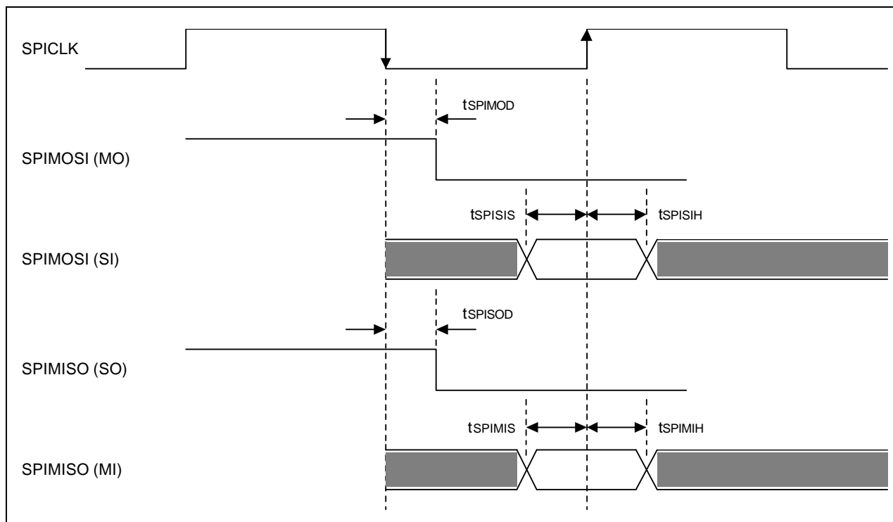
Figure 27-35. SPI Interface Timing Diagram (CPHA=1, CPOL=1)
