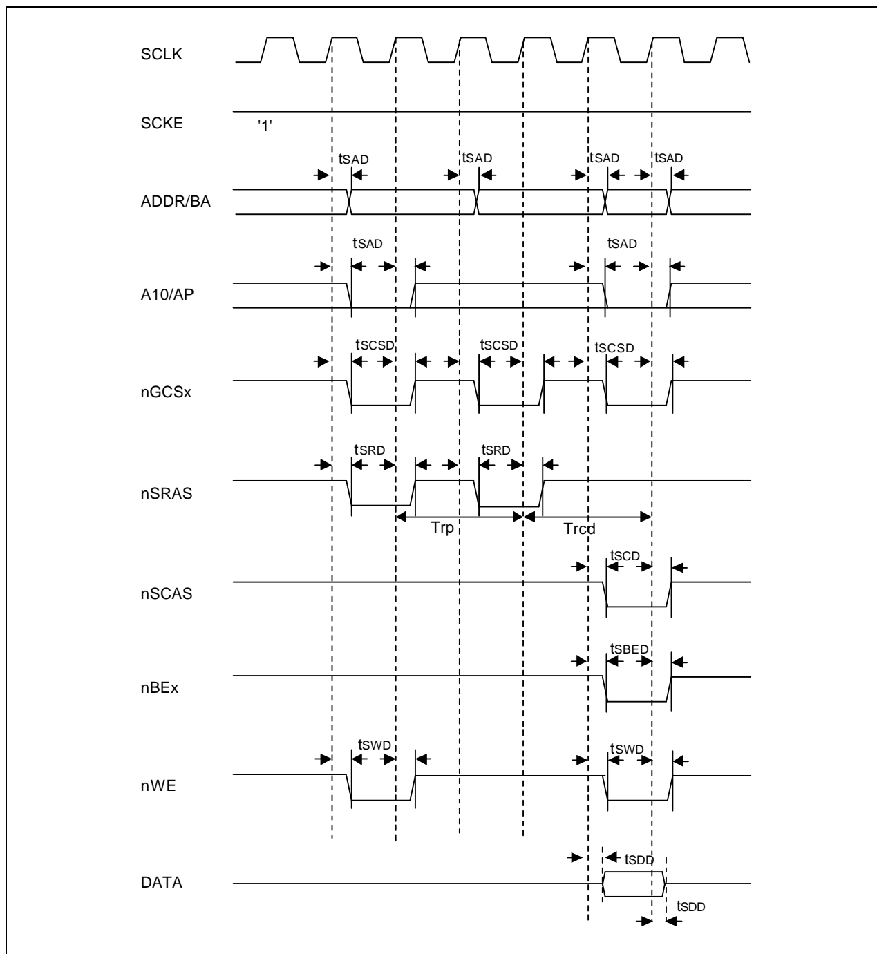
Figure 27-28. SDRAM Single Write Timing Diagram ( T_{rp}=2 , T_{rcd}=2 )
