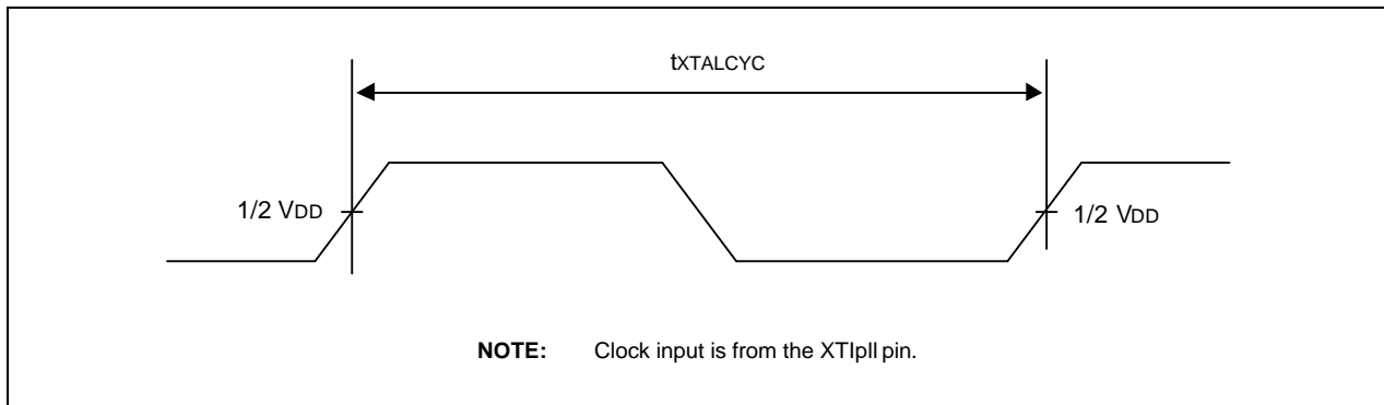
Figure 27-2. XTlpII Clock Timing Diagram
