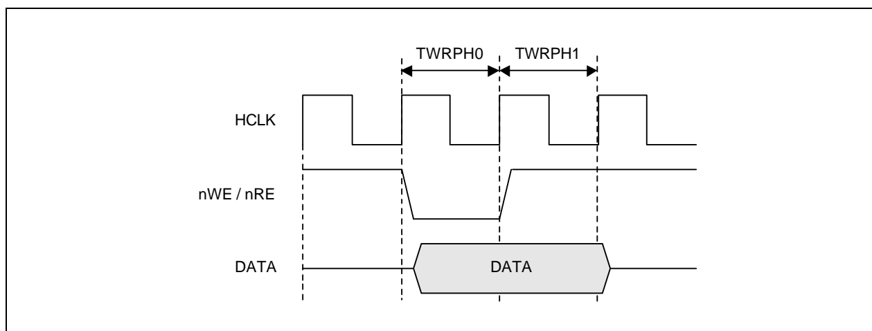
Figure 6-4. nWE &amp; nRE Timing (TWRPH0=0, TWRPH1=0)
