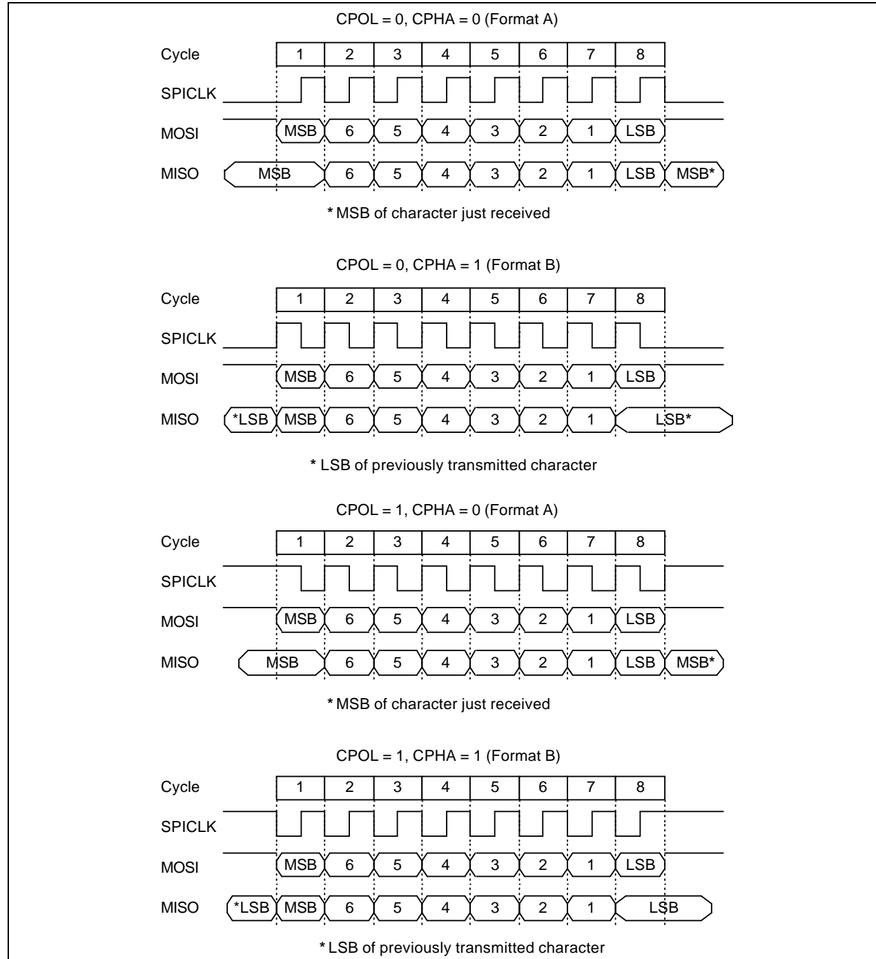
Figure 22-2. SPI Transfer Format
