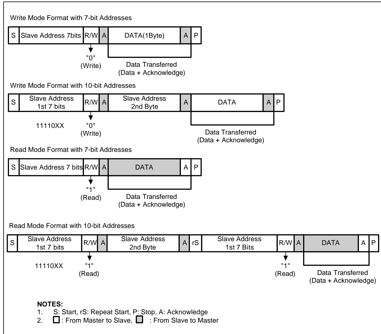
Figure 20-3. IIC-Bus Interface Data Format
