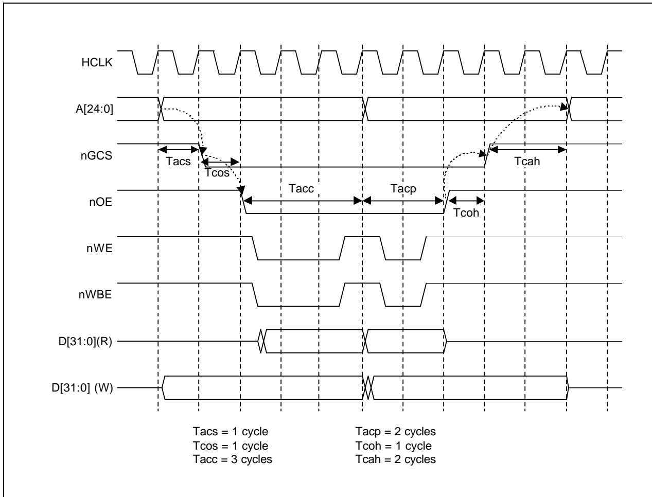
Figure 5-12. S3C2440A nGCS Timing Diagram
