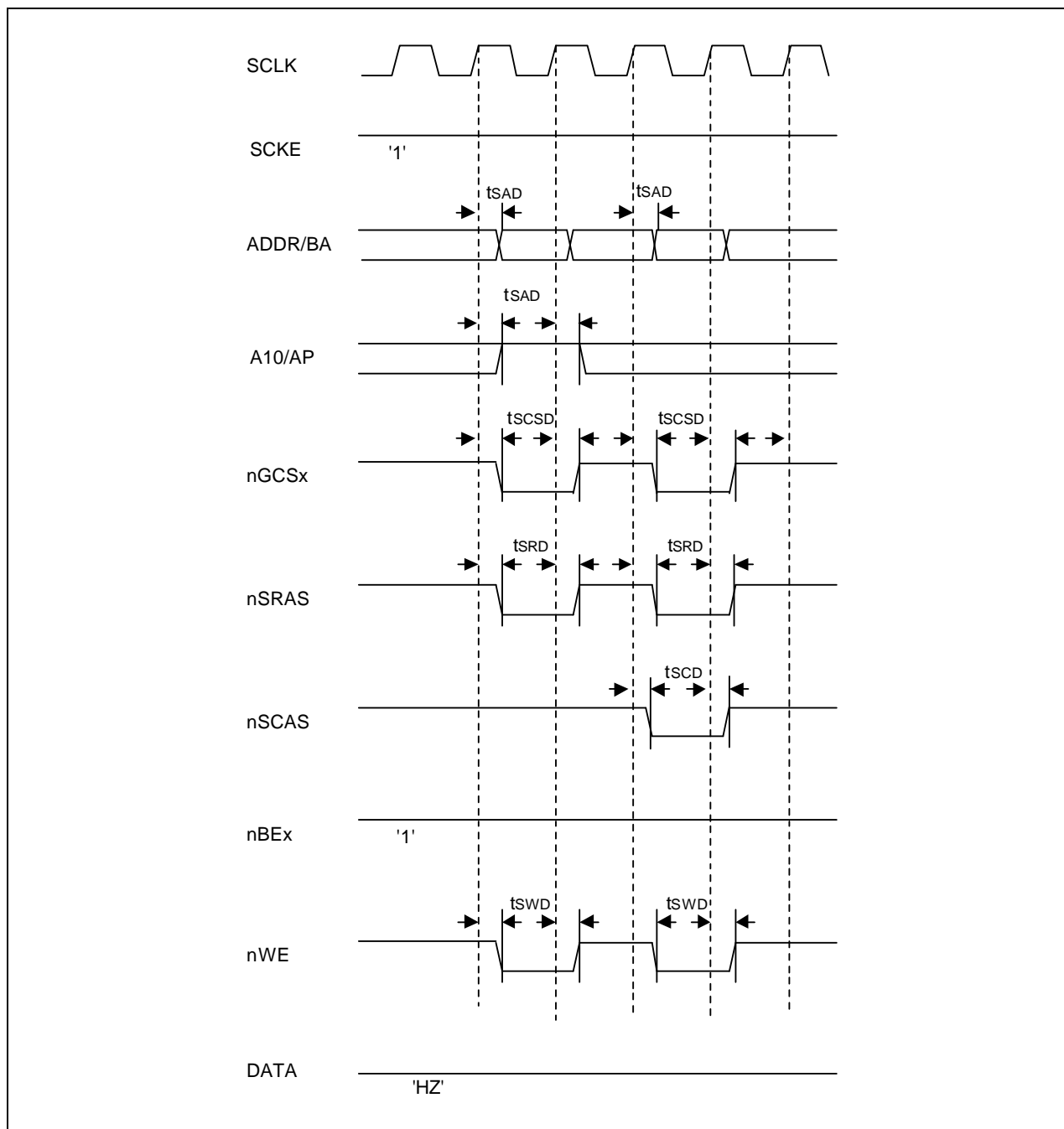
Figure 27-22. SDRAM MRS Timing Diagram
