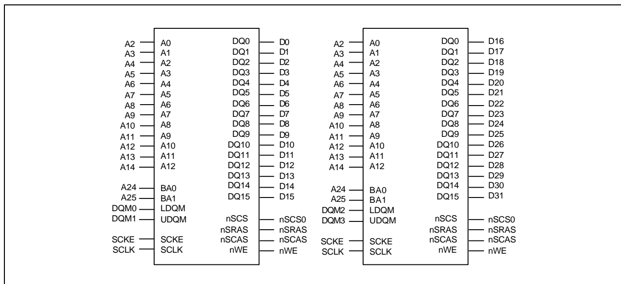
Figure 5-11. Memory Interface with 16-bit SDRAM (4Mx16x4Bank * 2ea)
