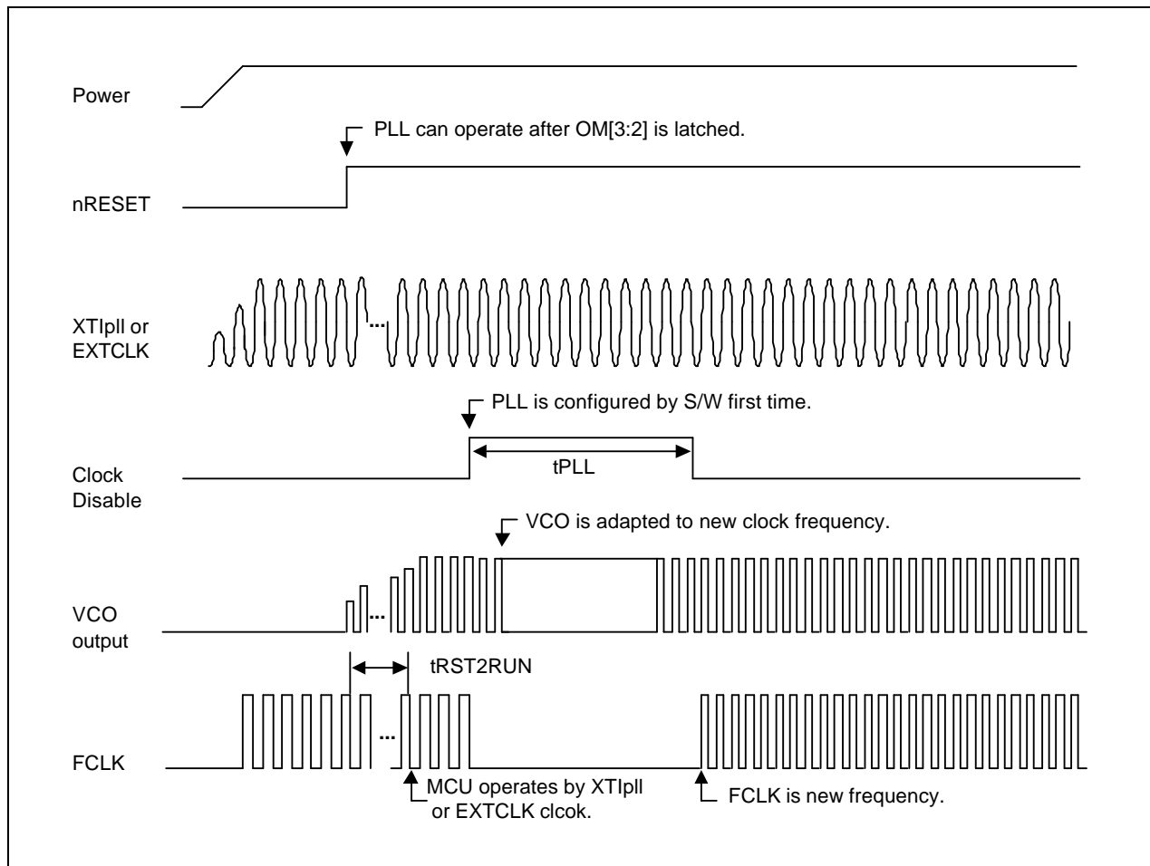
Figure 27-7. Power-On Oscillation Setting Timing Diagram
