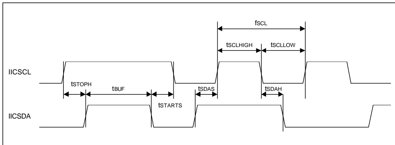
Figure 27-33. IIC Interface Timing Diagram
