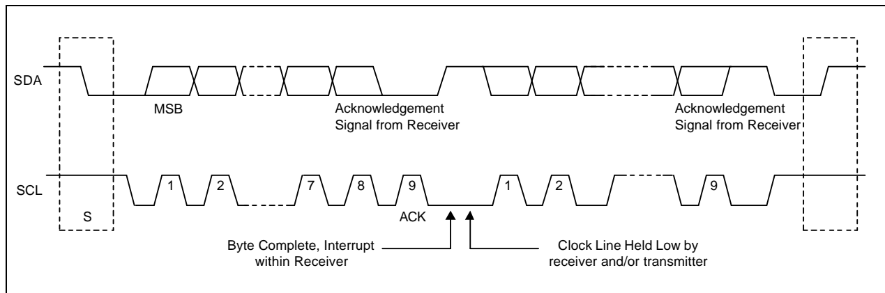
Figure 20-4. Data Transfer on the IIC-Bus
