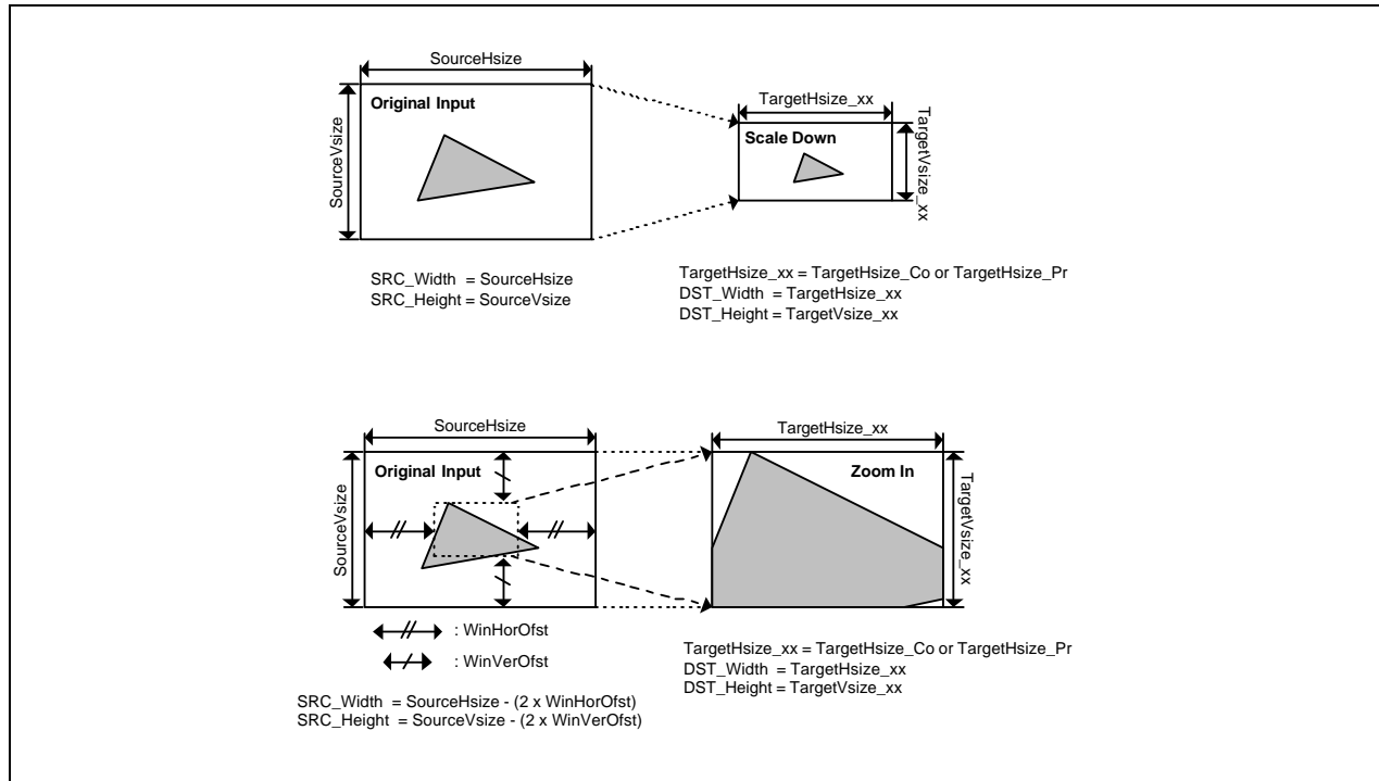
Figure 23-12. Scaling Scheme
