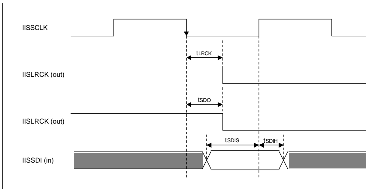
Figure 27-32. IIS Interface Timing Diagram
