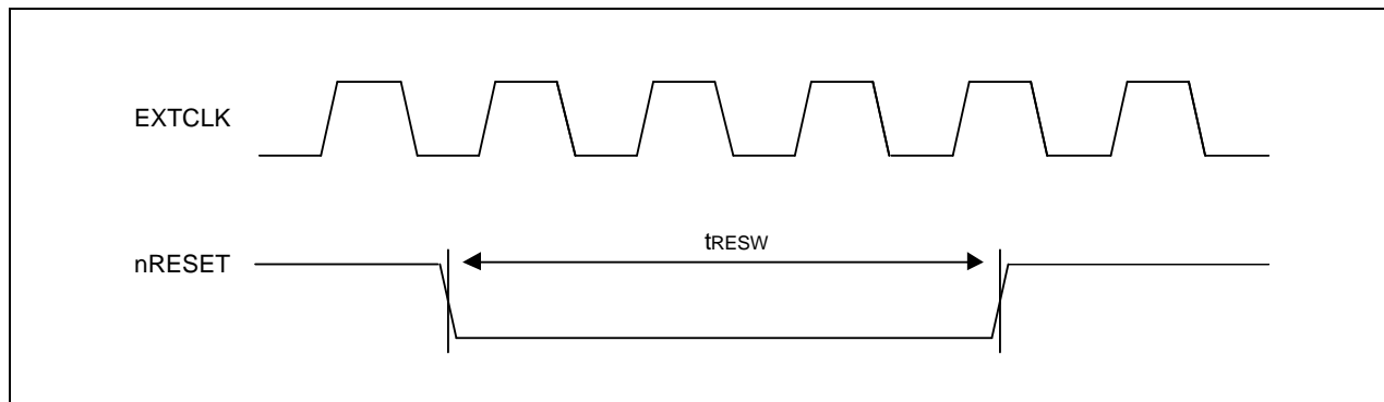
Figure 27-6. Manual Reset Input Timing Diagram
