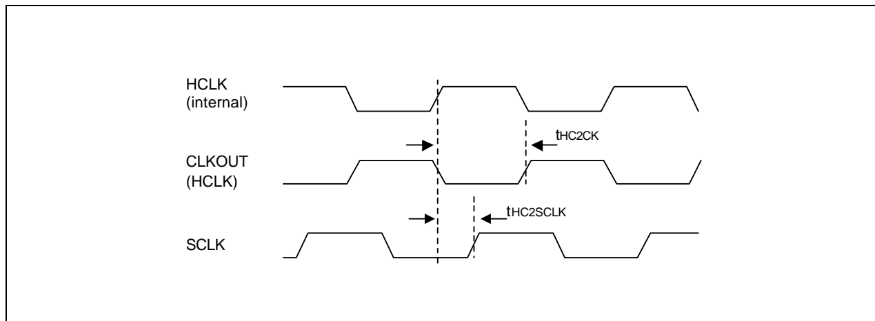
Figure 27-5. HCLK/CLKOUT/SCLK in case when EXTCLK is used
