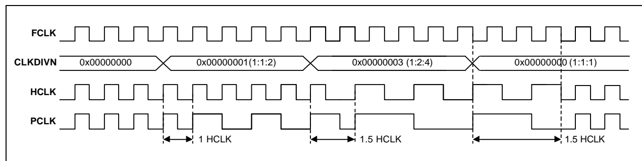
Figure 7-6. Example of Internal Clock Change
