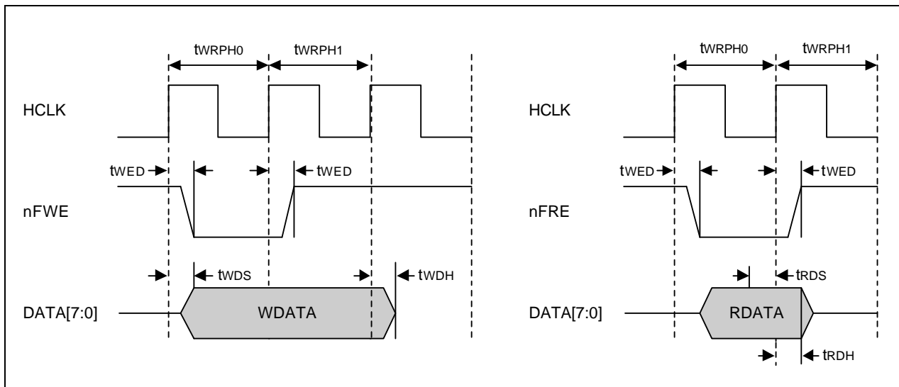
Figure 27-37. NAND Flash Timing Diagram
