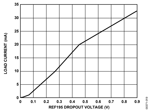
Figure 19. Load Current vs. REF195 Dropout Voltage
