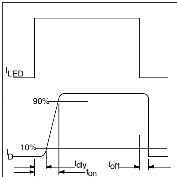
Figure 7. Delay Time Definitions
