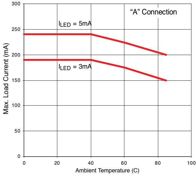
Figure 1. Current Derating Curves
