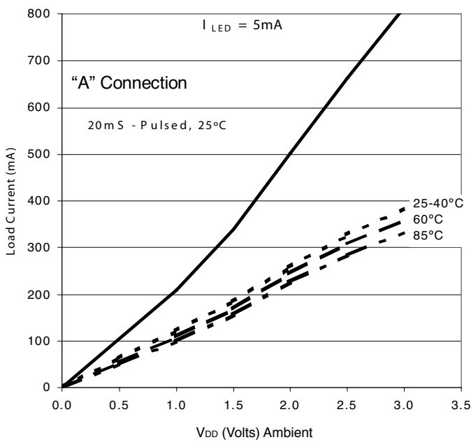
Figure 3. Typical On-Characteristics
