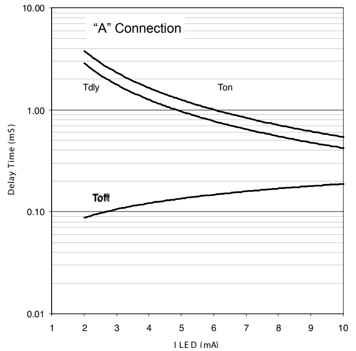
Figure 6. Typical Delay Times
