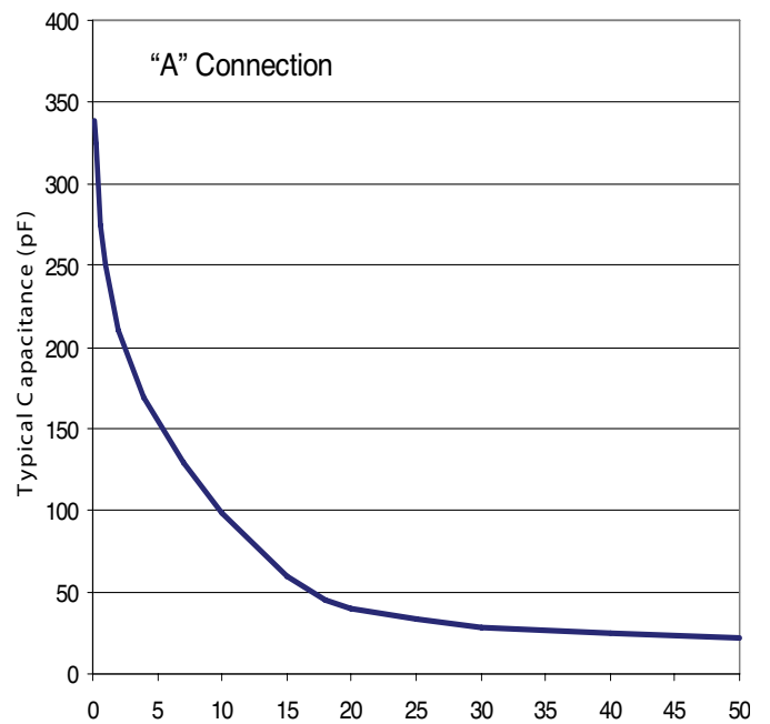
Figure 8. Typical Output Capacitance
