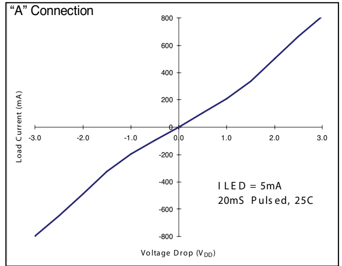
Figure 2. Typical On Characteristics
