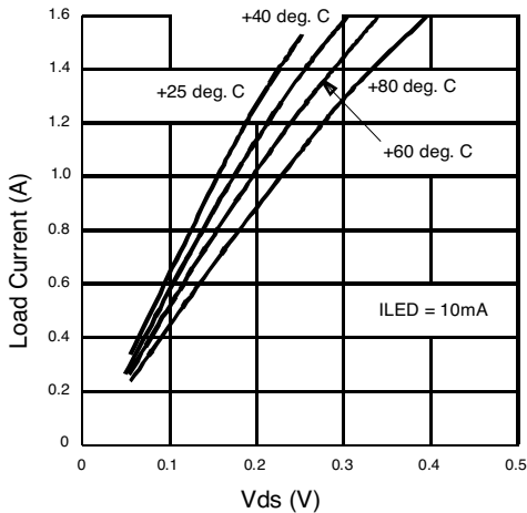
Figure 3. Typical On-Characteristics
