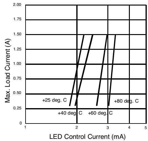
Figure 2. Typical Control Current Requirements
