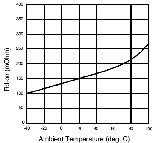
Figure 4. Typical On-Resistance
