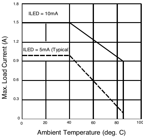
Figure 1. Current Derating Curves
