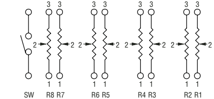
SCHEMATIC
