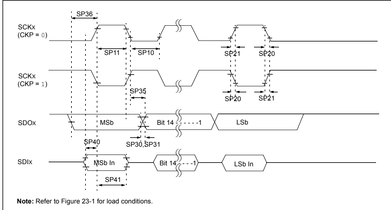
FIGURE 23-10: SPIx MODULE MASTER MODE (CKE = 1) TIMING CHARACTERISTICS
