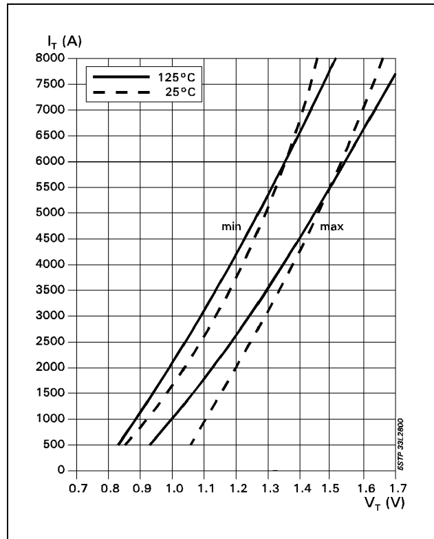
Fig. 3 On-state characteristics.
