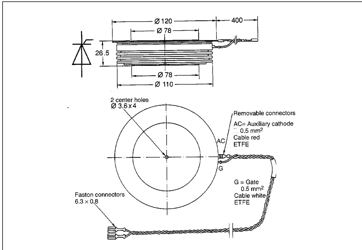
Fig. 12 Device Outline Drawing.
