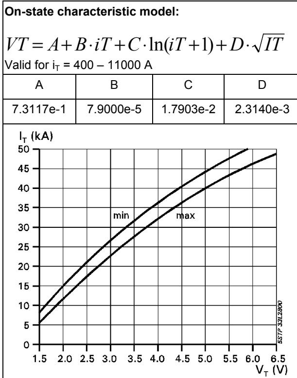
Fig. 2 On-state characteristics. T_j = 125^\circ\text{C} , 10ms half sine
