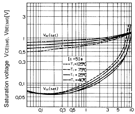
Base and Collector Saturation Voltage
