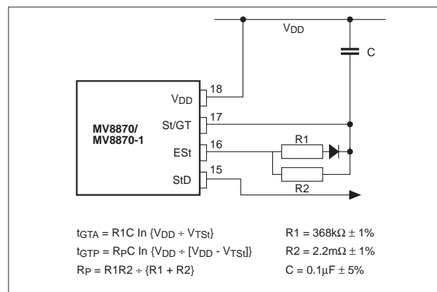
Figure 12: Non-symmetric guard time circuit
