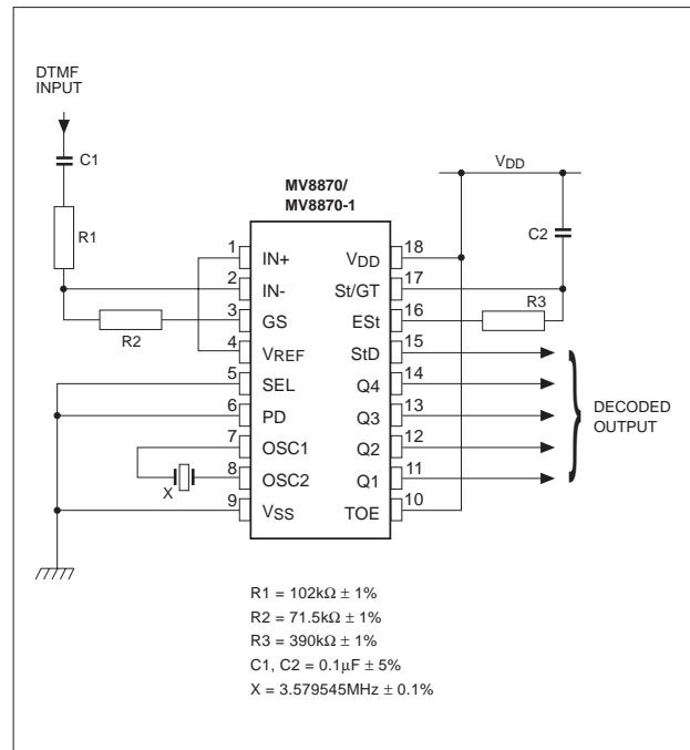
Figure 11: Single ended circuit for BT/CEPT Specs
