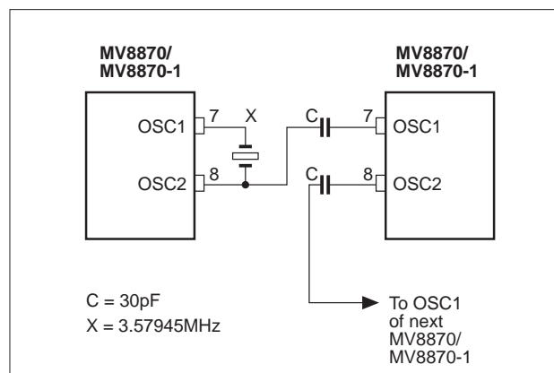
Figure 10: Oscillator circuit
