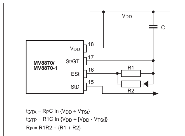
Figure 8b: Guard time adjustment ( t_{GTP} > t_{GTA} )
