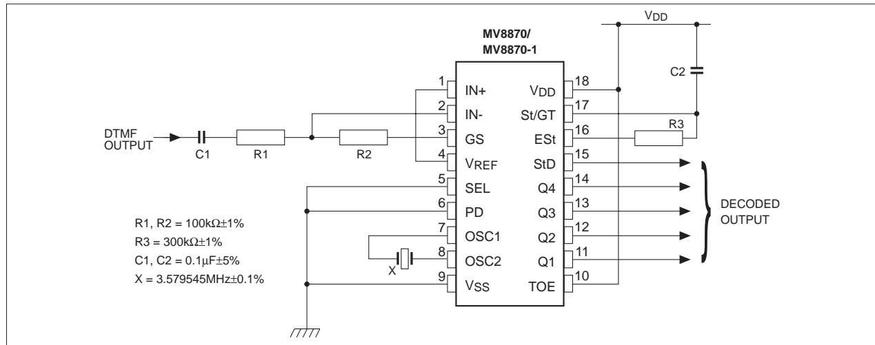
Figure 7: Simple application circuit; single ended input
