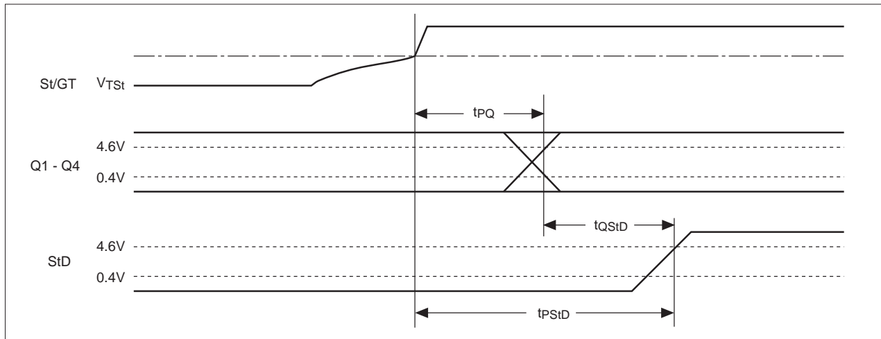
Figure 14: Timing - decoded data
