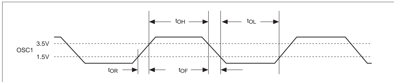
Figure 13: Timing - external oscillator input
