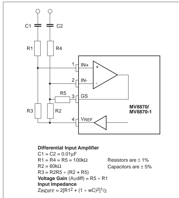
Figure 9: Differential input configuration
