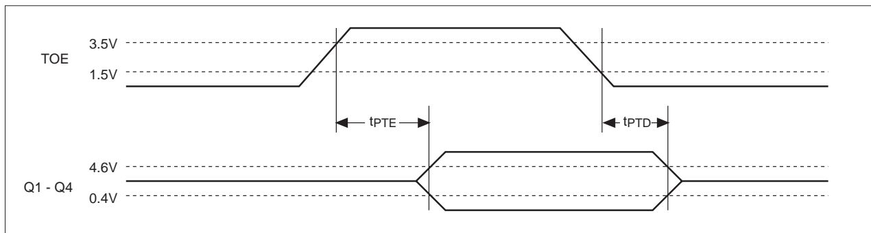
Figure 15: Timing - Output enable and disable
