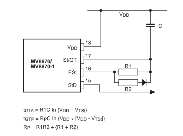
Figure 8a: Guard time adjustment ( t_{GTP} < t_{GTA} )
