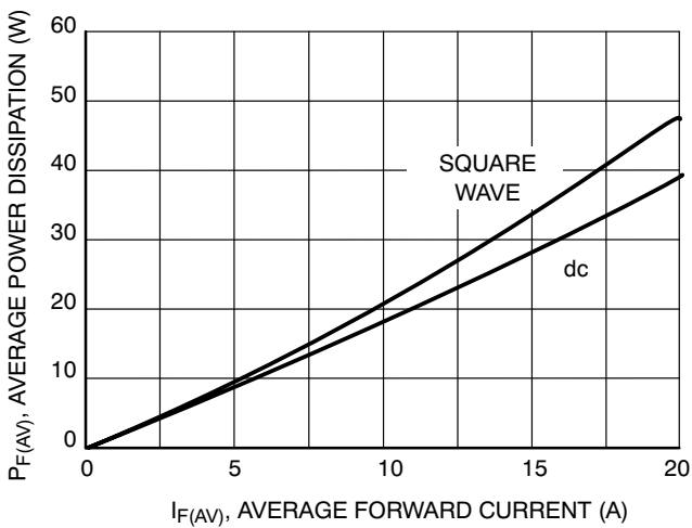
Figure 4. Power Dissipation
