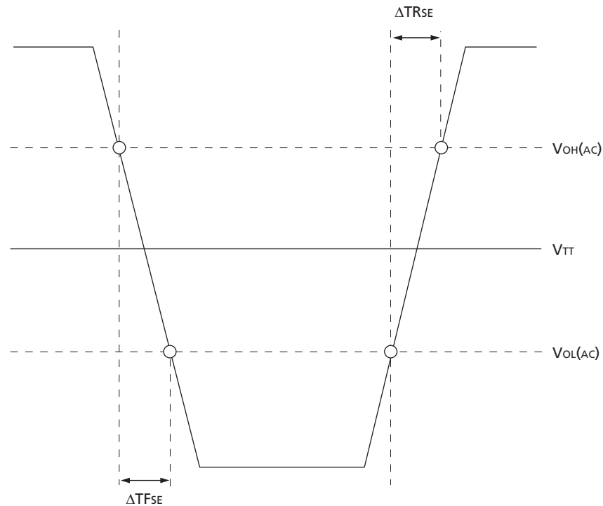
Figure 32: Nominal Slew Rate Definition for Single-Ended Output Signals
