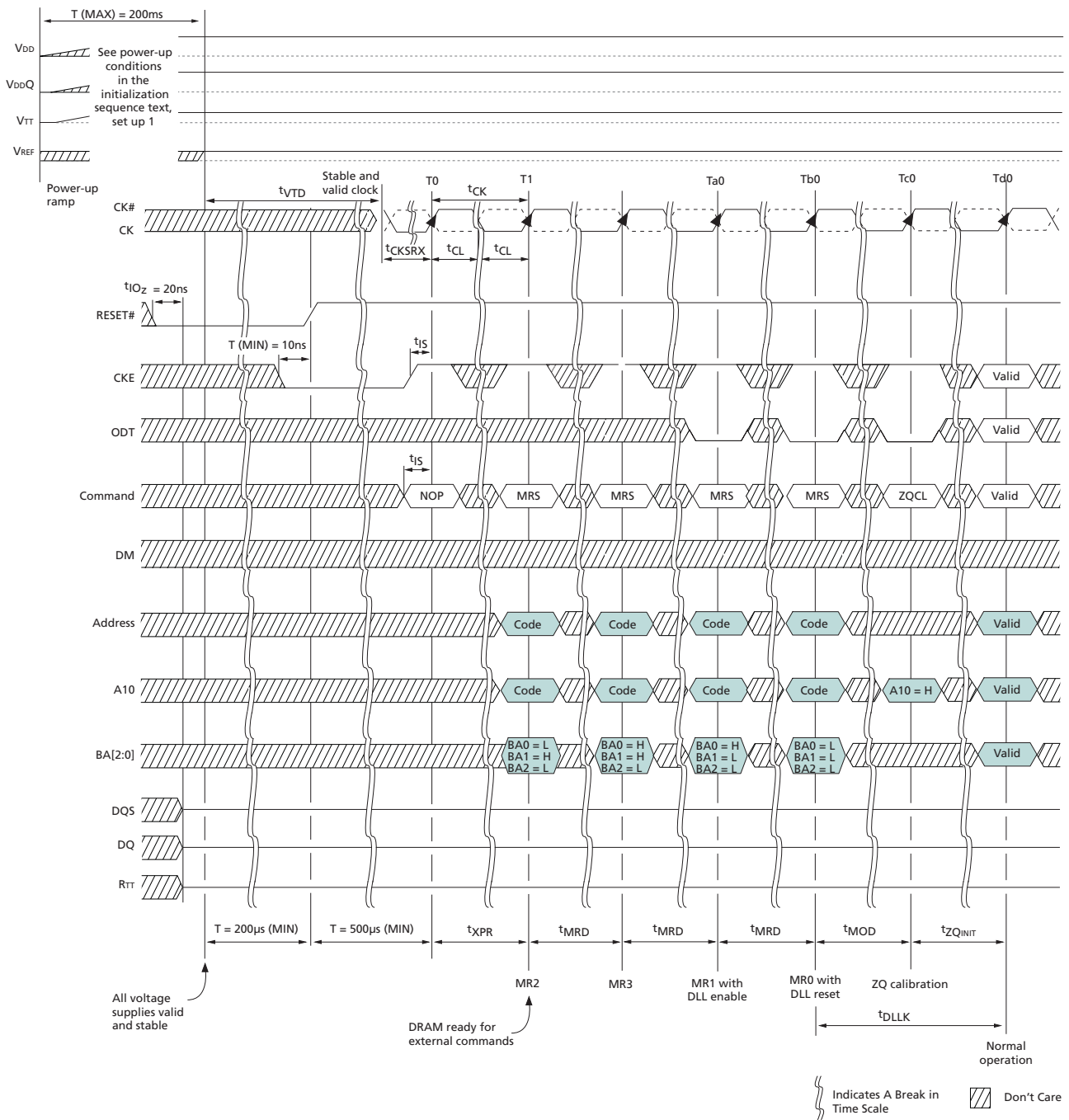
Figure 50: Initialization Sequence
