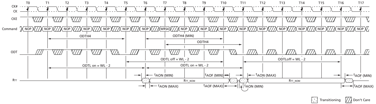
Figure 116: Synchronous ODT (BC4)
