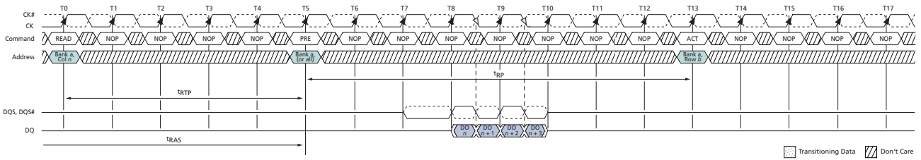
Figure 76: READ to PRECHARGE (AL = 5, CL = 6)
