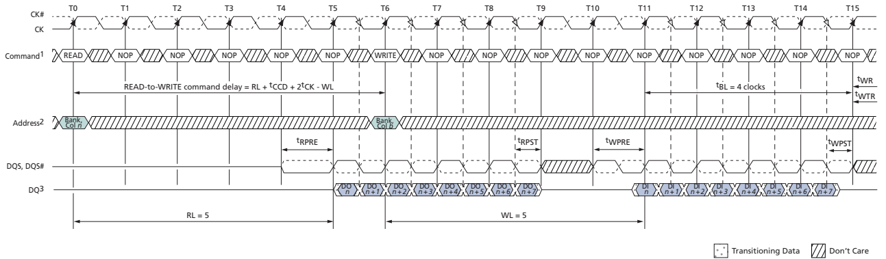
Figure 72: READ (BL8) to WRITE (BL8)
