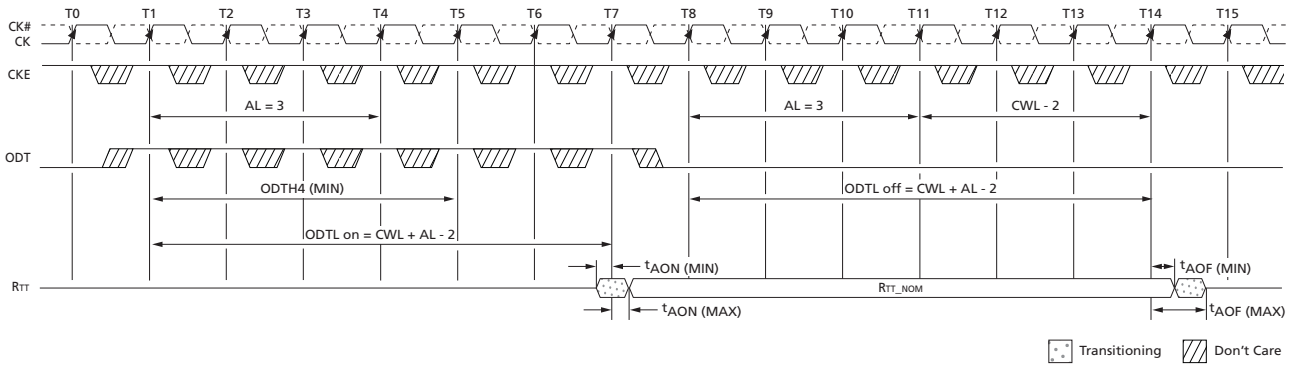
Figure 115: Synchronous ODT
