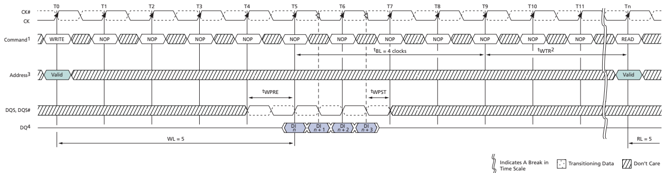
Figure 91: WRITE (BC4 OTF) to READ (BC4 OTF)
